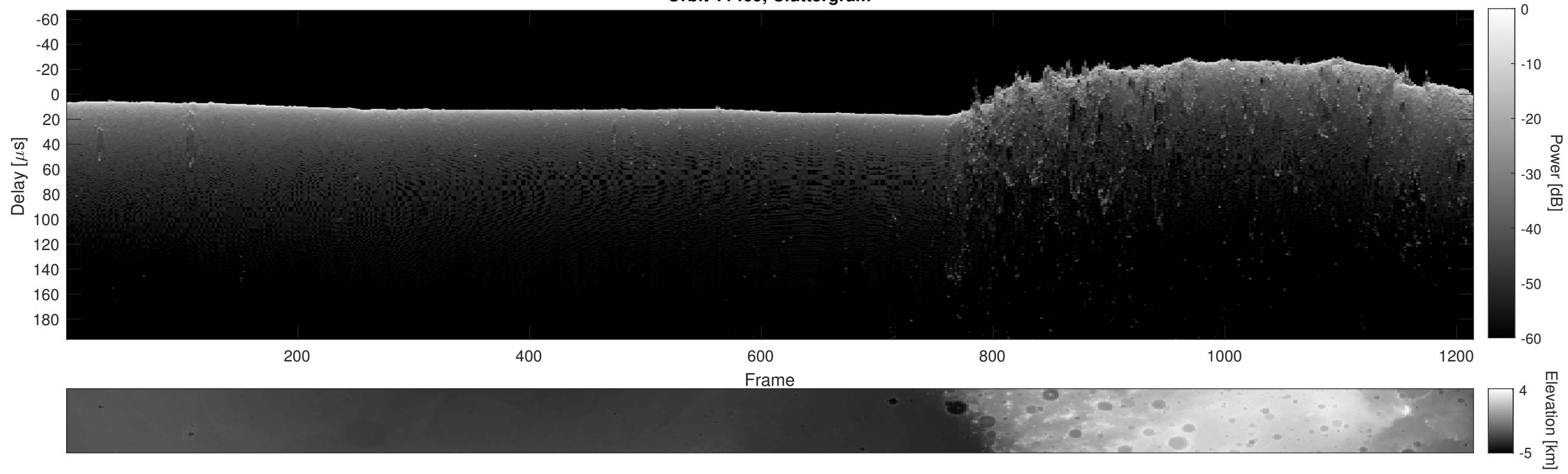
Orbit 11469, Cluttergram
