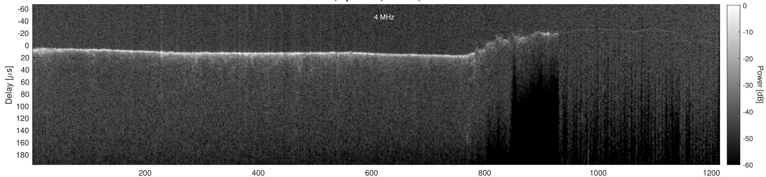
Orbit 11469, Cluttergram
