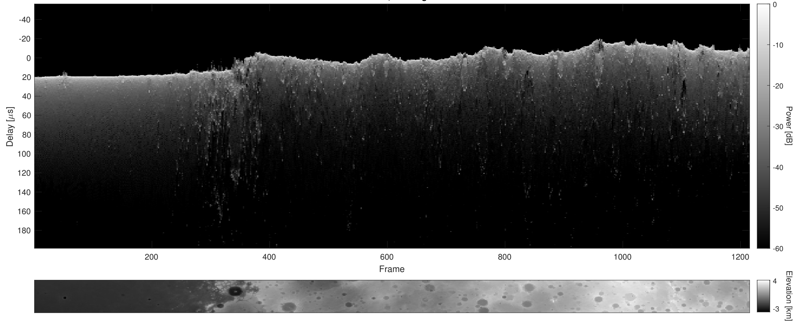
Orbit 11473, Cluttergram
