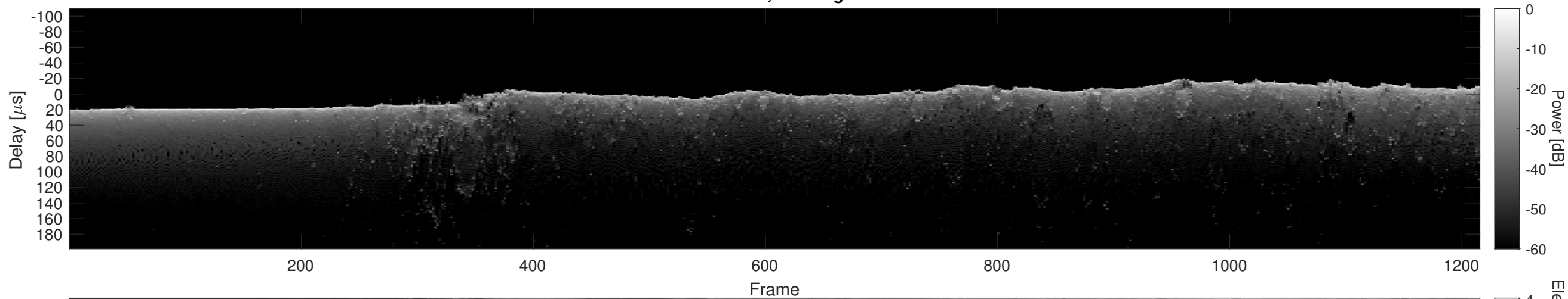
Orbit 11473, Cluttergram
