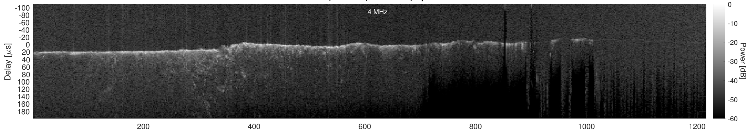
Orbit 11473, Cluttergram
