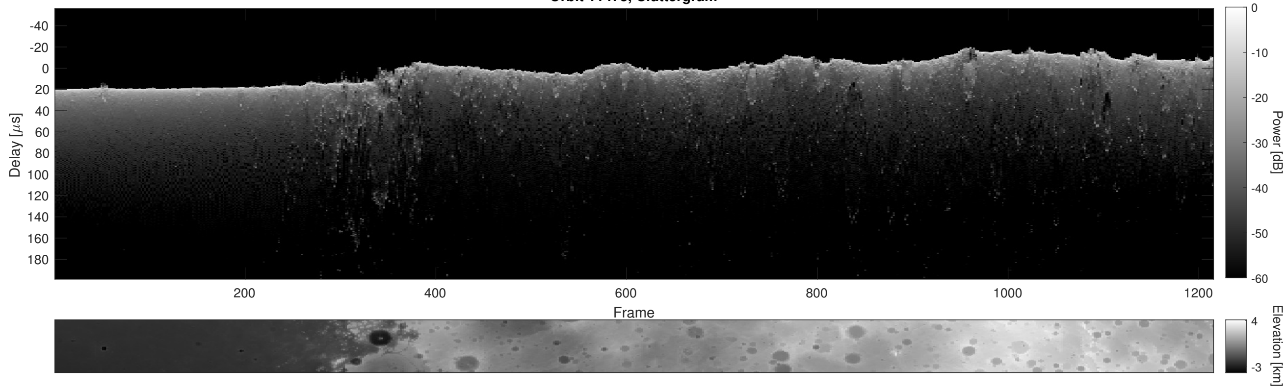
Orbit 11473, Cluttergram
