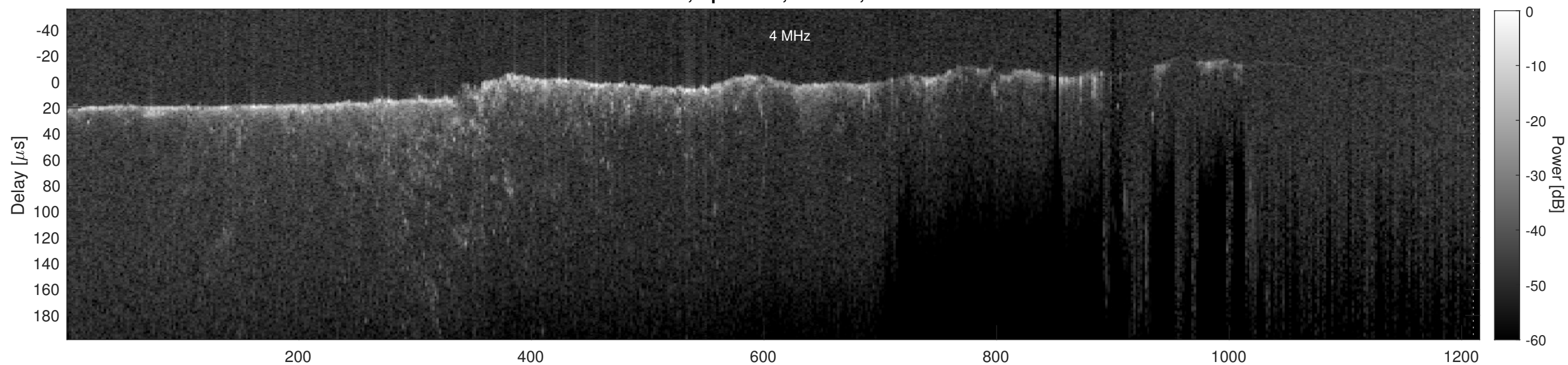
Orbit 11473, Cluttergram
