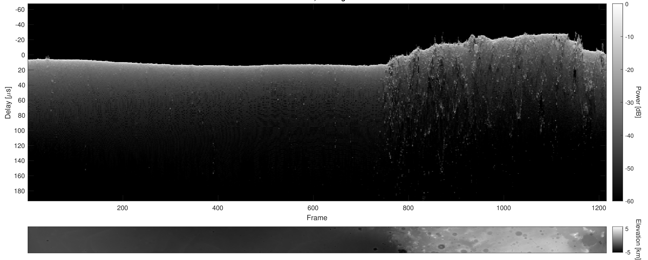
Orbit 11476, Cluttergram
