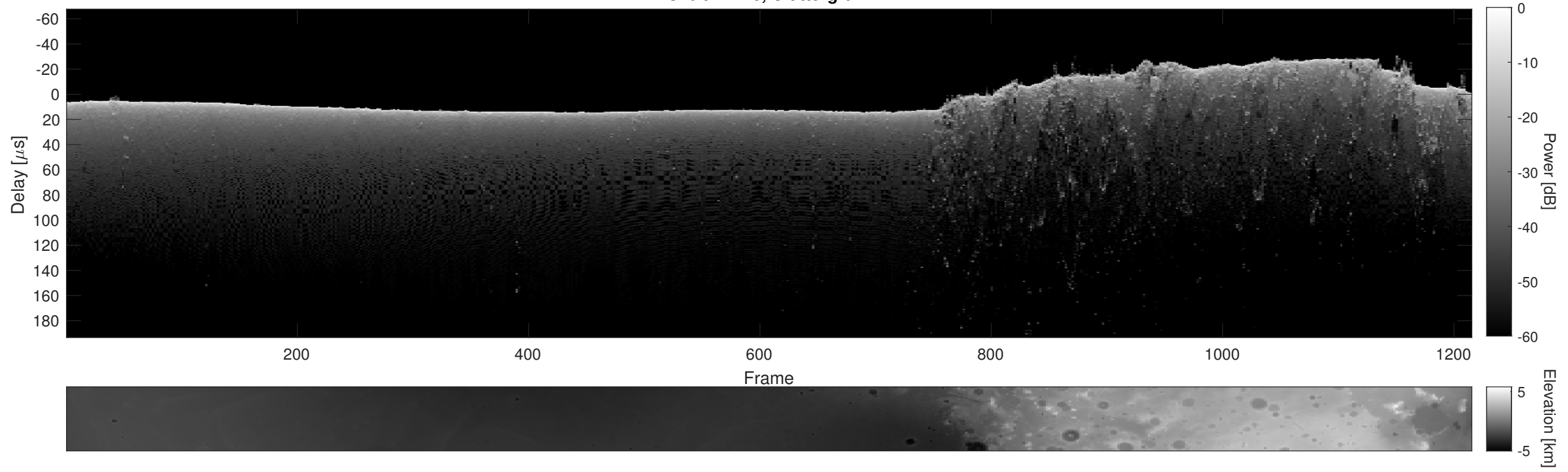
Orbit 11476, Cluttergram
