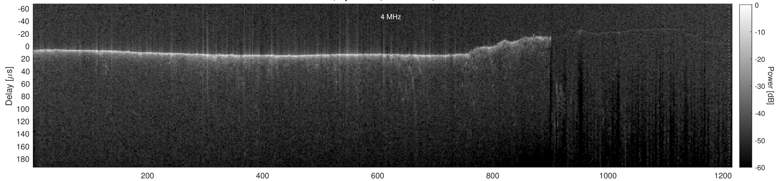
Orbit 11476, Cluttergram
