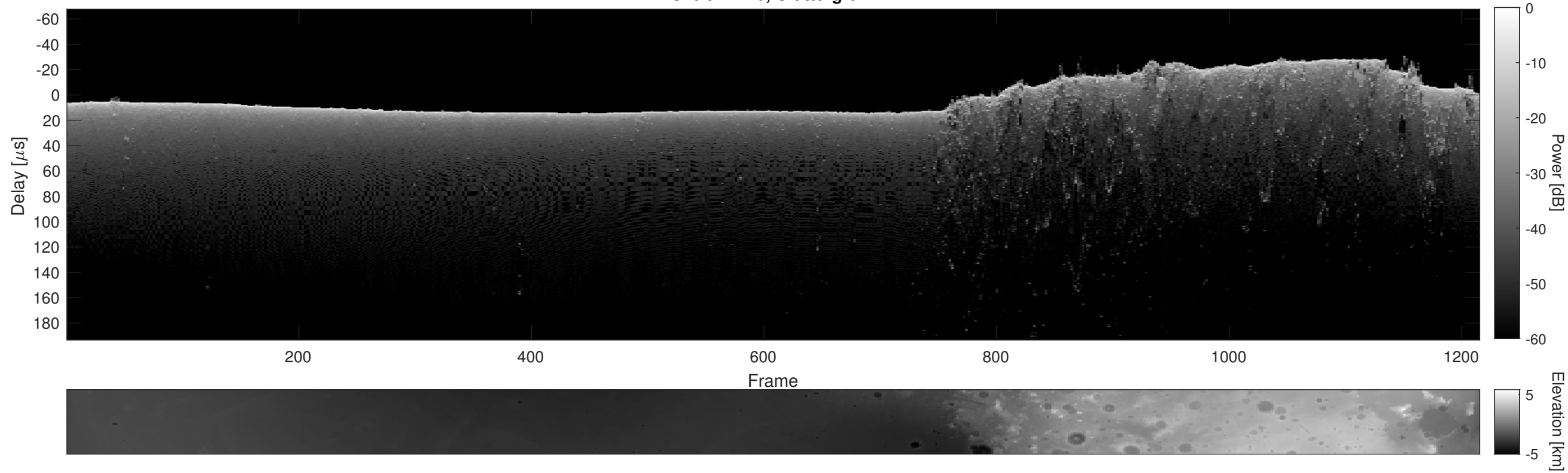
Orbit 11476, Cluttergram
