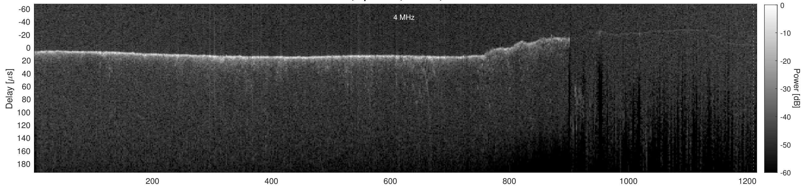
Orbit 11476, Cluttergram
