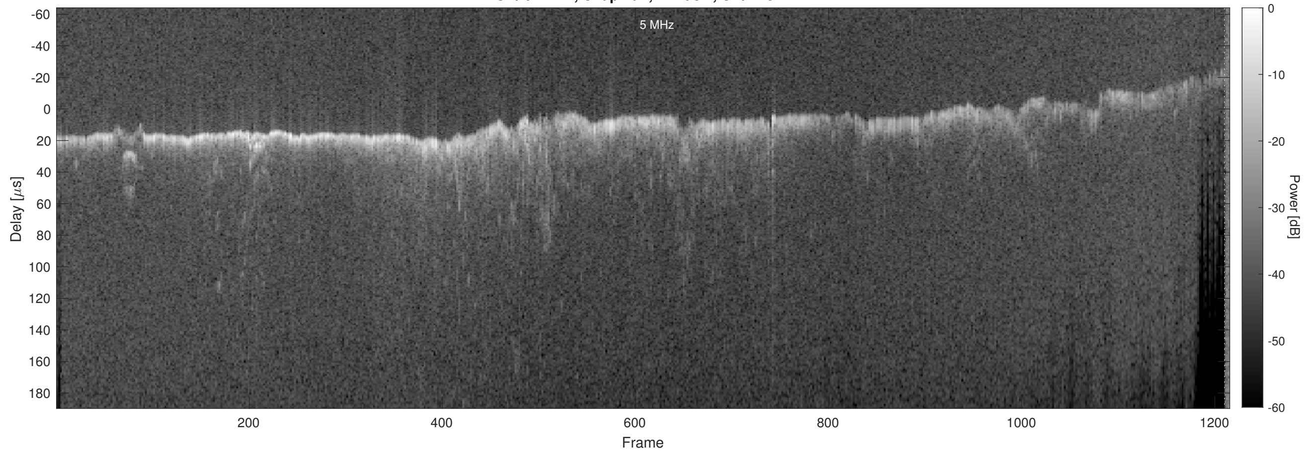
Orbit 11477, Chapman, Window, Channel 2
