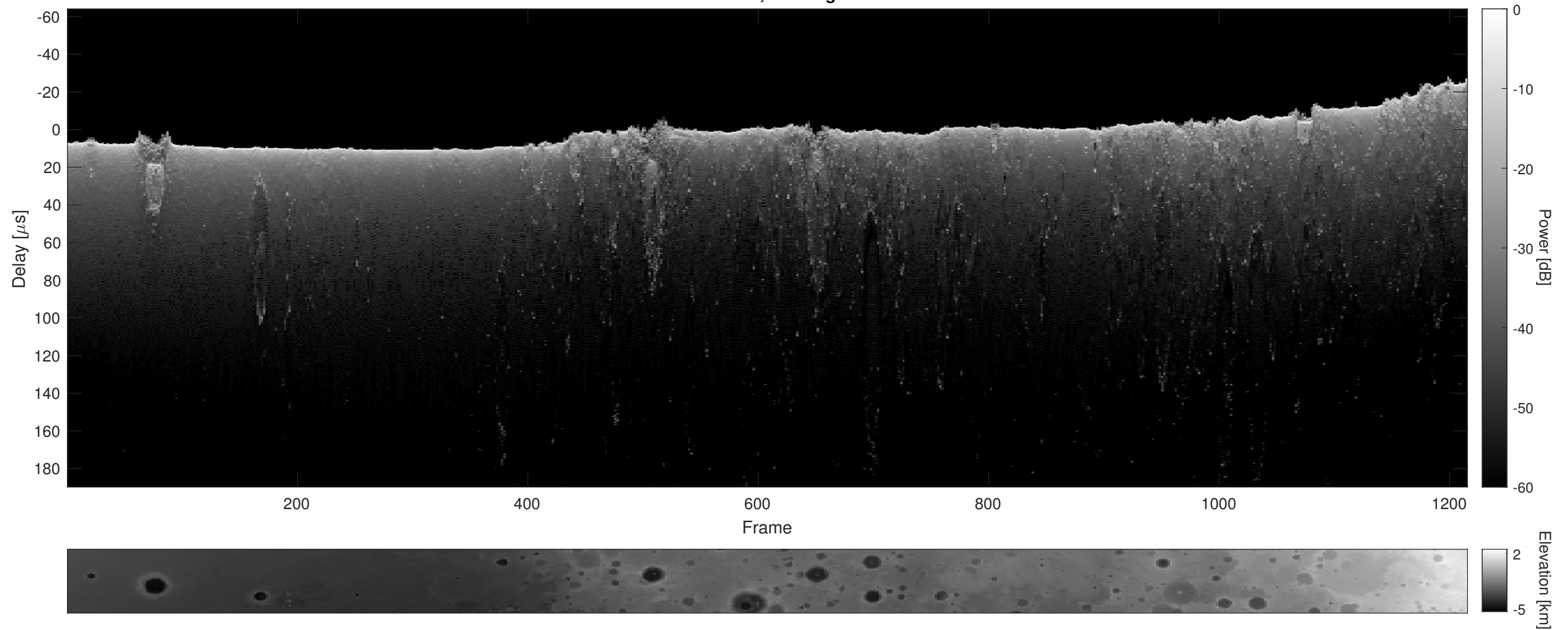
Orbit 11477, Cluttergram
