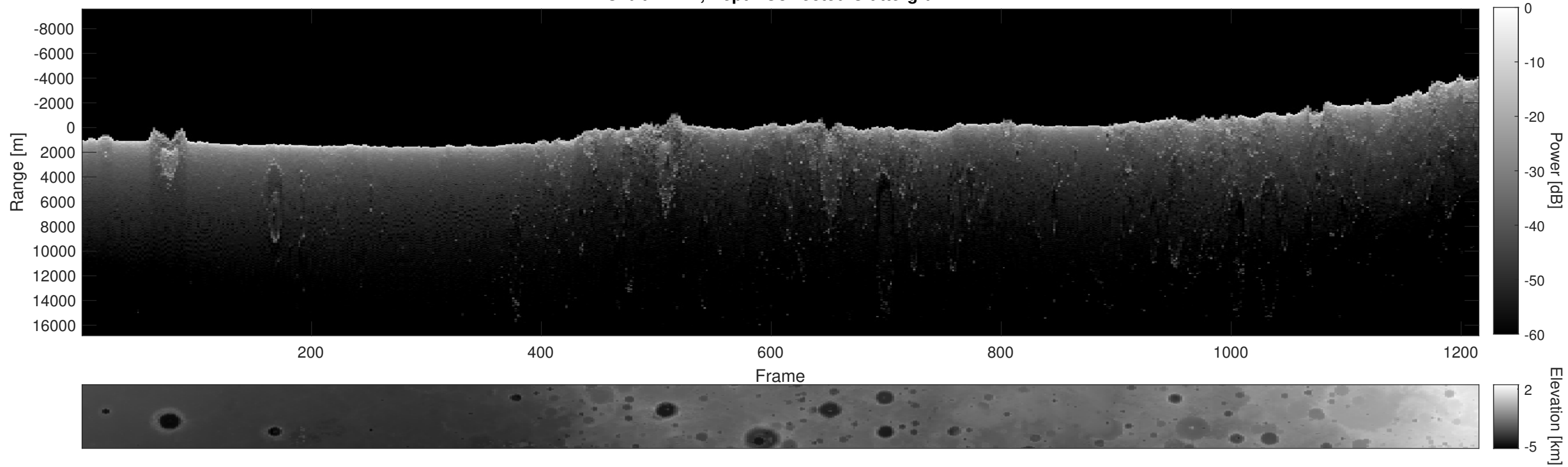
Orbit 11477, Depth-Corrected Cluttergram
