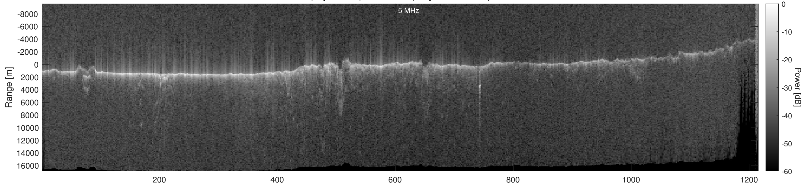
Orbit 11477, Optimized, No Window, Depth-Corrected, Channel 2
