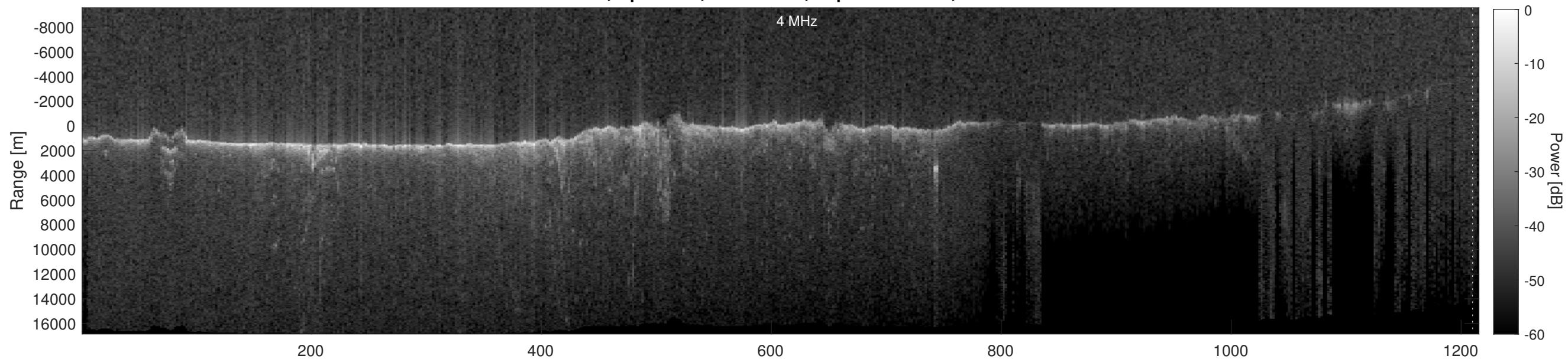
Orbit 11477, Depth-Corrected Cluttergram
