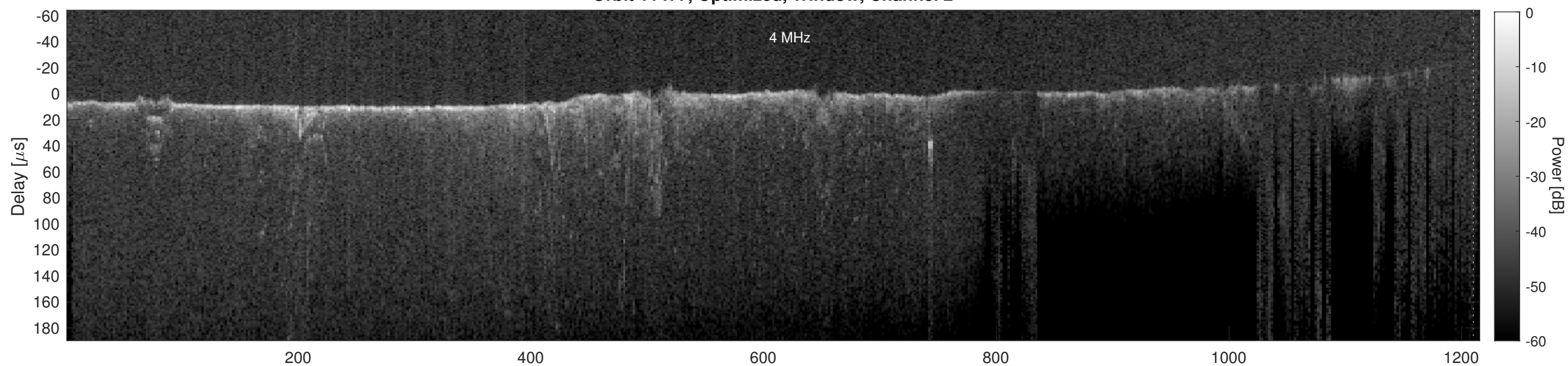
Orbit 11477, Cluttergram
