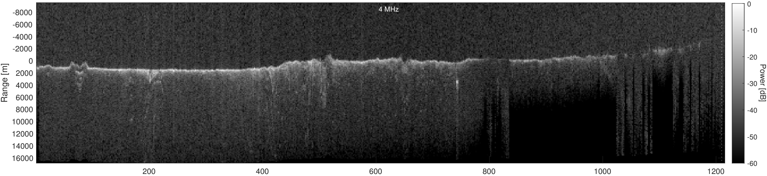
Orbit 11477, Depth-Corrected Cluttergram
