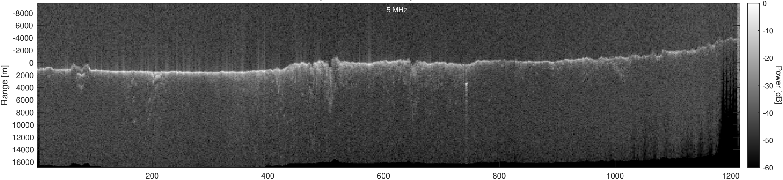
Orbit 11477, Optimized, Window, Depth-Corrected, Channel 2
