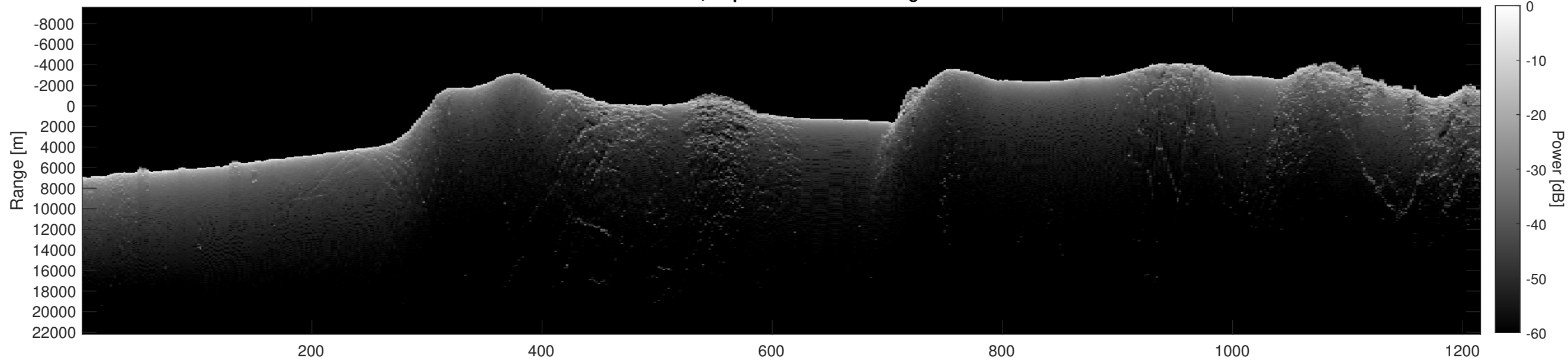
Orbit 11478, Depth-Corrected Cluttergram
