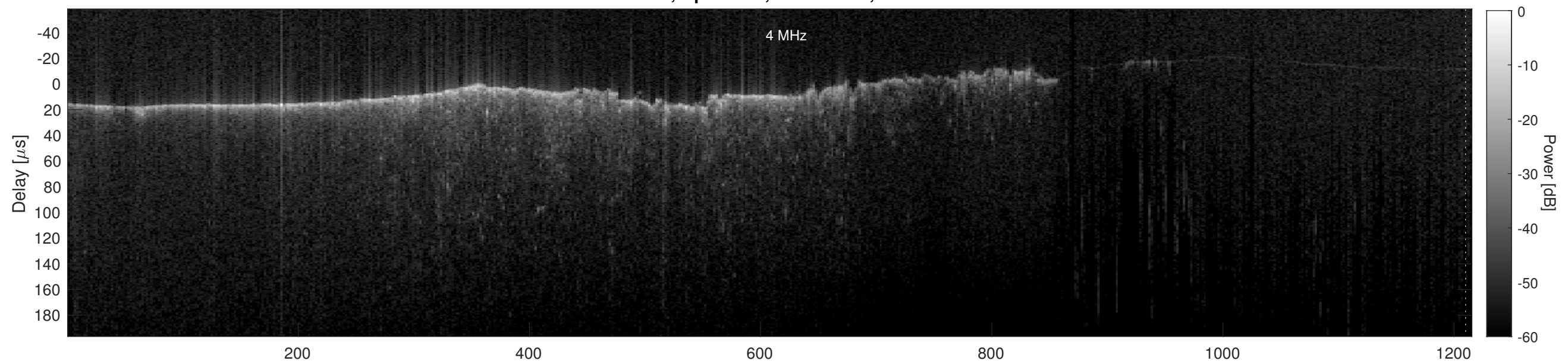
Orbit 11481, Cluttergram
