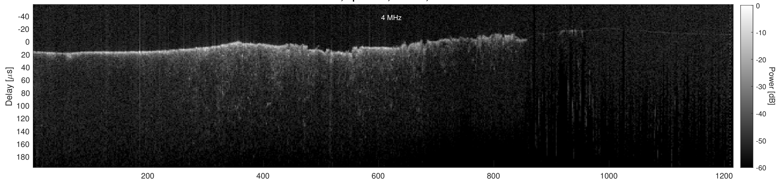
Orbit 11481, Cluttergram
