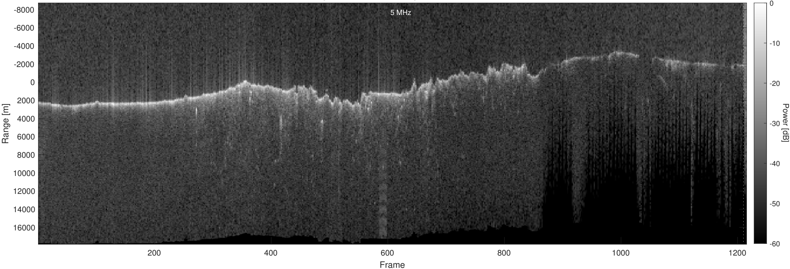
Orbit 11481, Optimized, Window, Depth-Corrected, Channel 2
