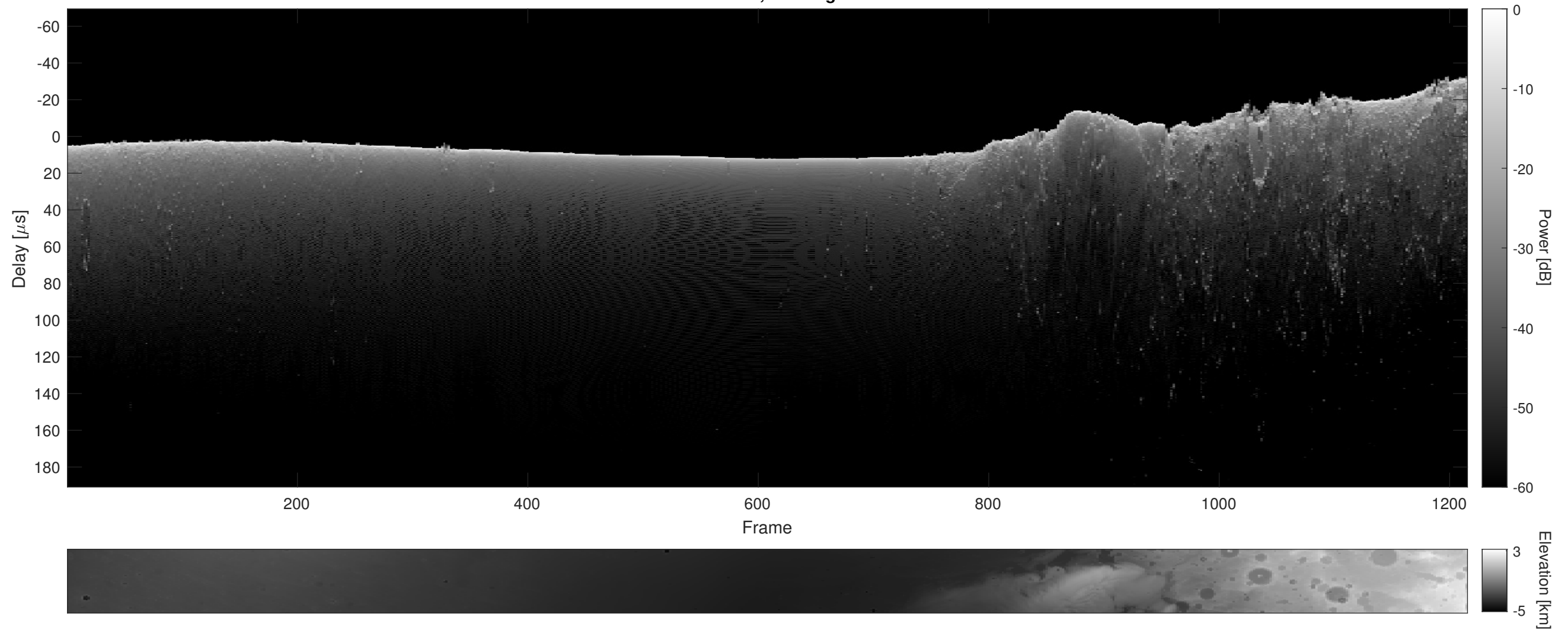
Orbit 11482, Cluttergram
