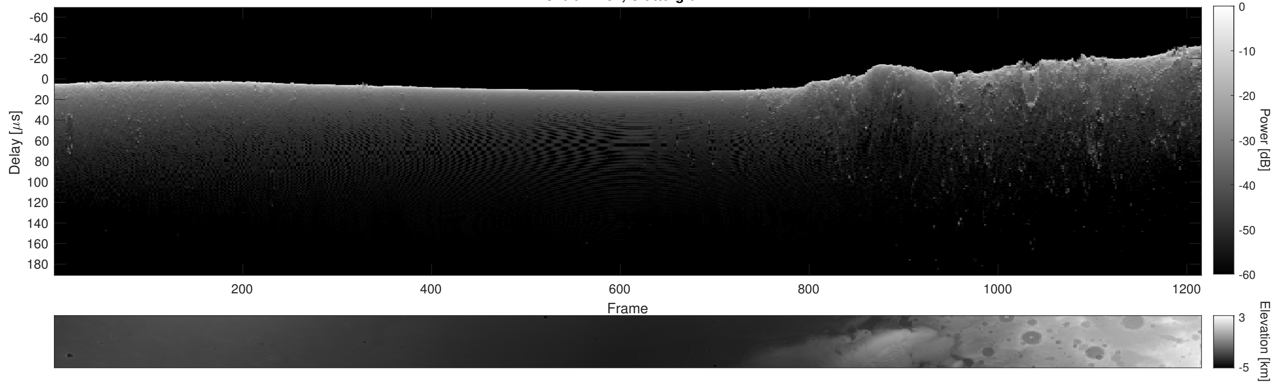
Orbit 11482, Cluttergram
