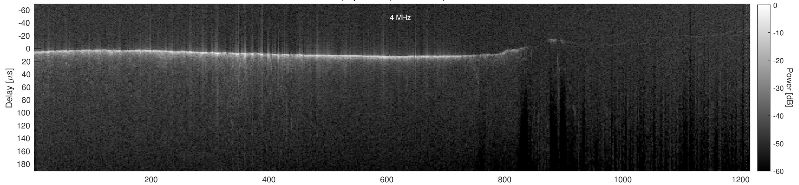
Orbit 11482, Cluttergram
