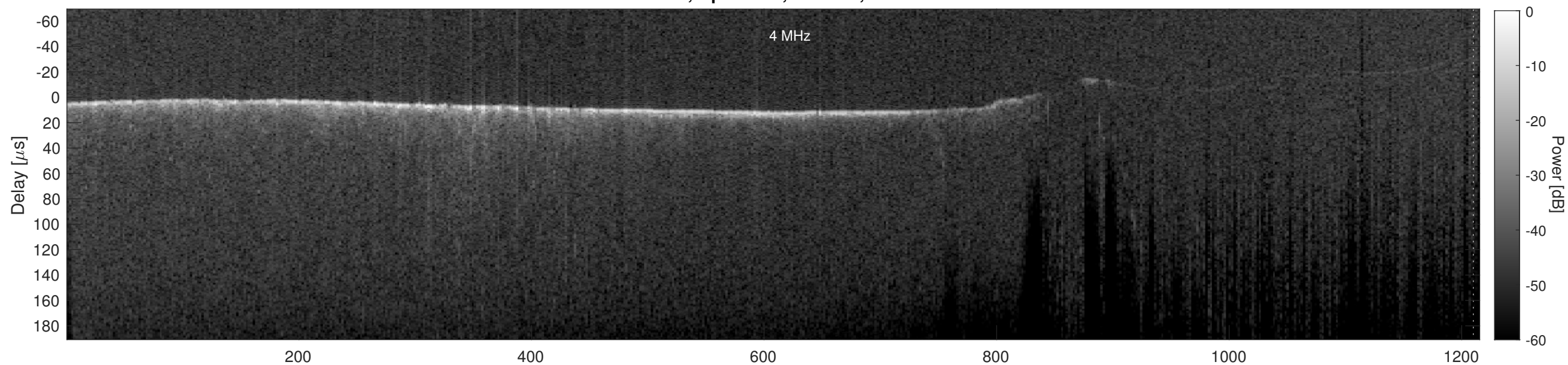
Orbit 11482, Cluttergram
