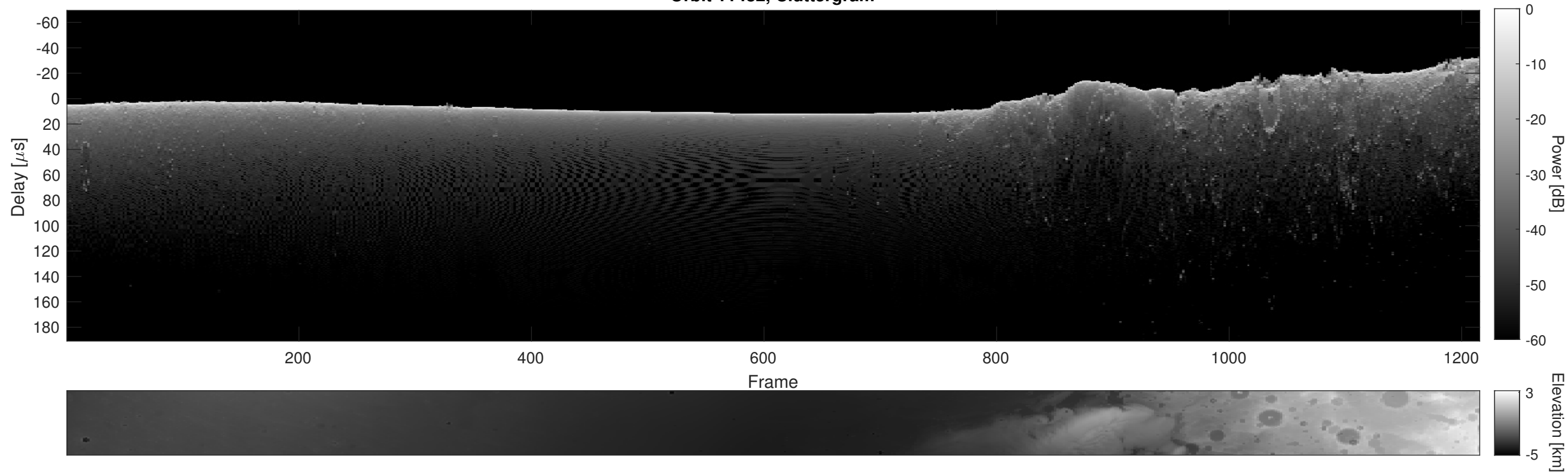
Orbit 11482, Cluttergram
