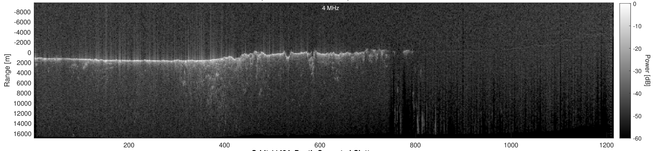
Orbit 11484, Depth-Corrected Cluttergram
