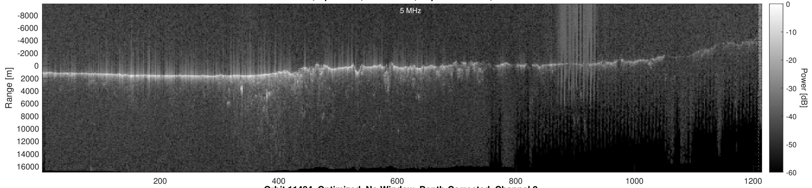
Orbit 11484, Optimized, No Window, Depth-Corrected, Channel 2
