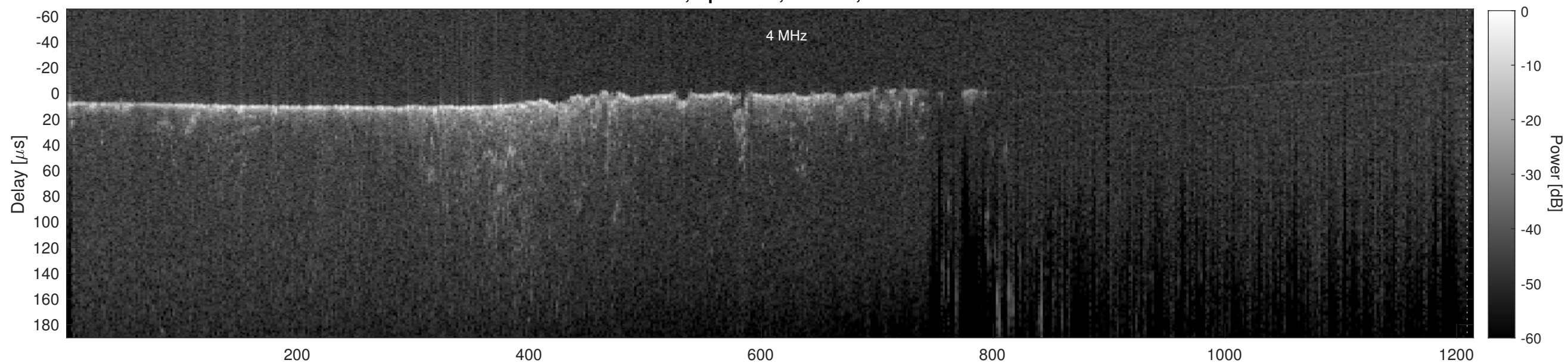
Orbit 11484, Cluttergram
