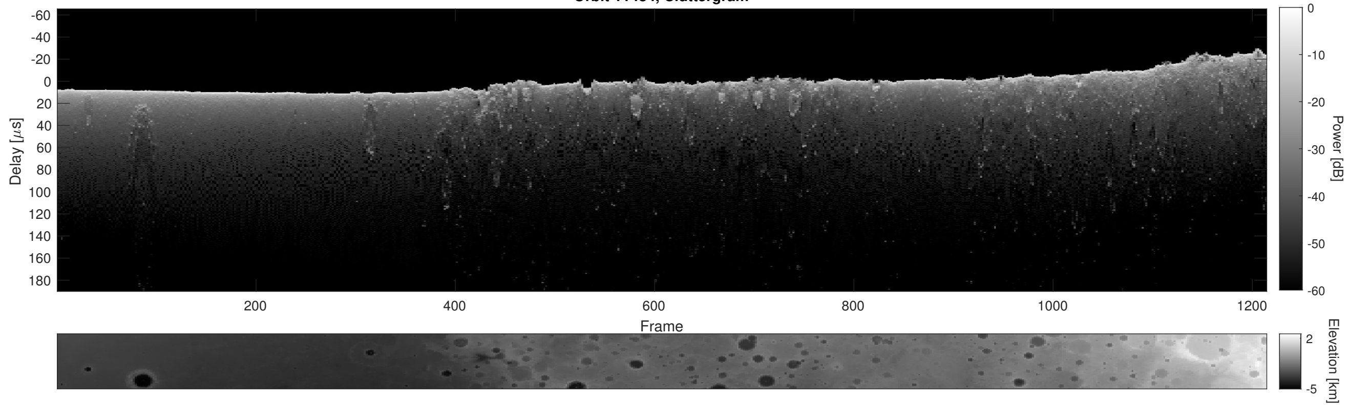
Orbit 11484, Cluttergram
