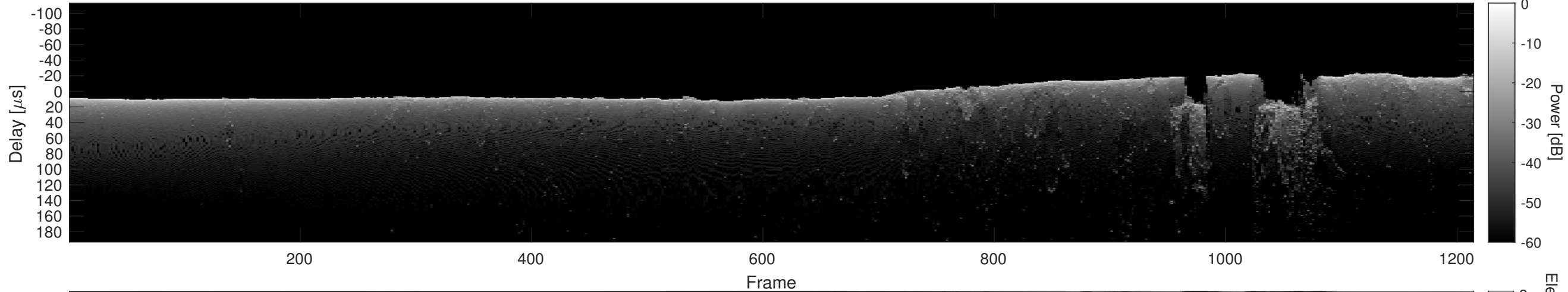
Orbit 11488, Cluttergram
