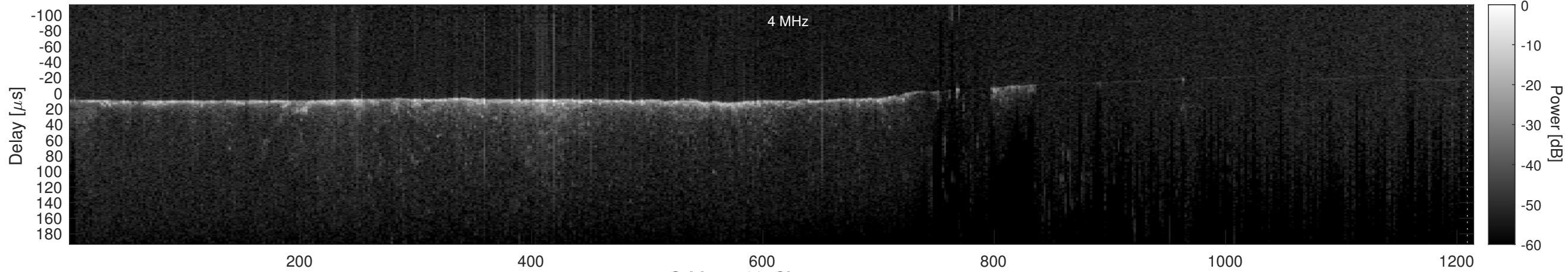
Orbit 11488, Cluttergram
