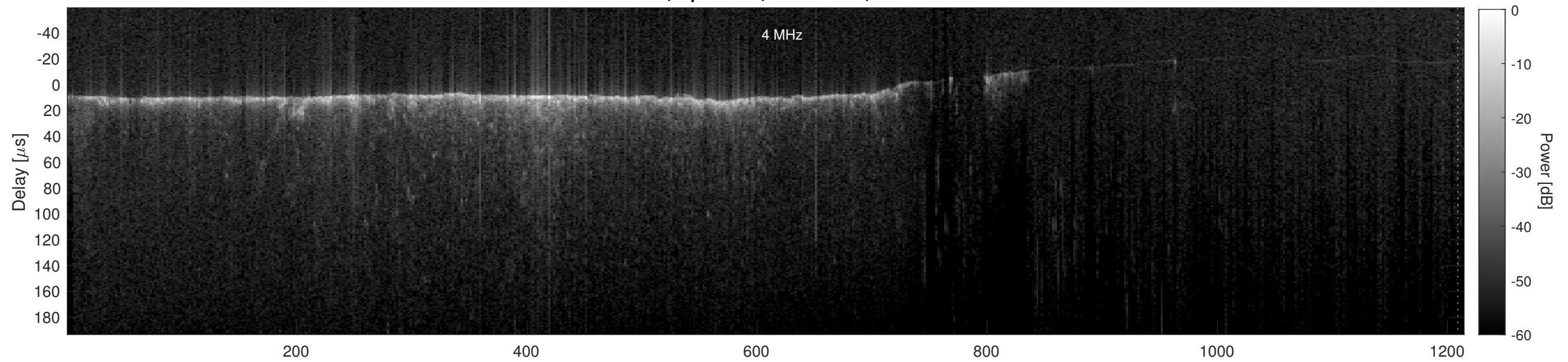
Orbit 11488, Cluttergram
