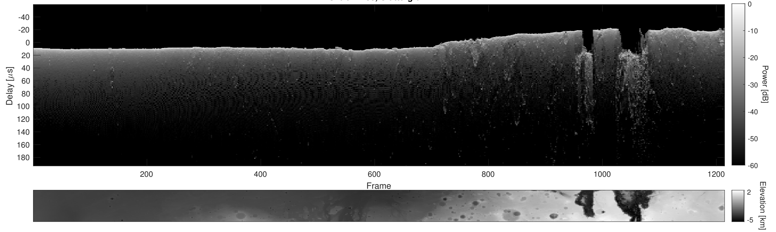
Orbit 11488, Cluttergram
