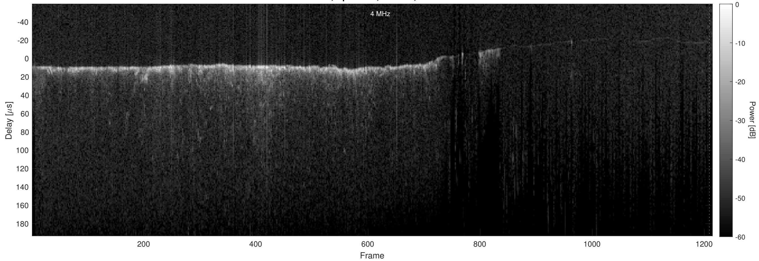
Orbit 11488, Optimized, Window, Channel 2
