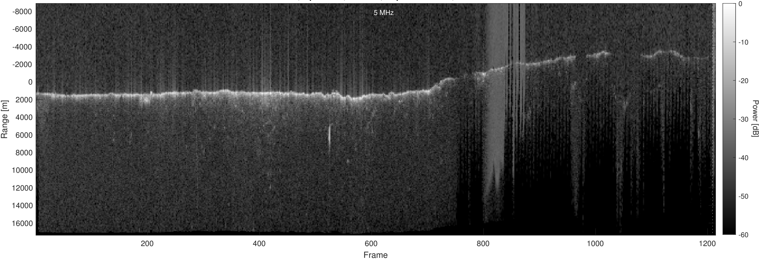
Orbit 11488, Optimized, Window, Depth-Corrected, Channel 2
