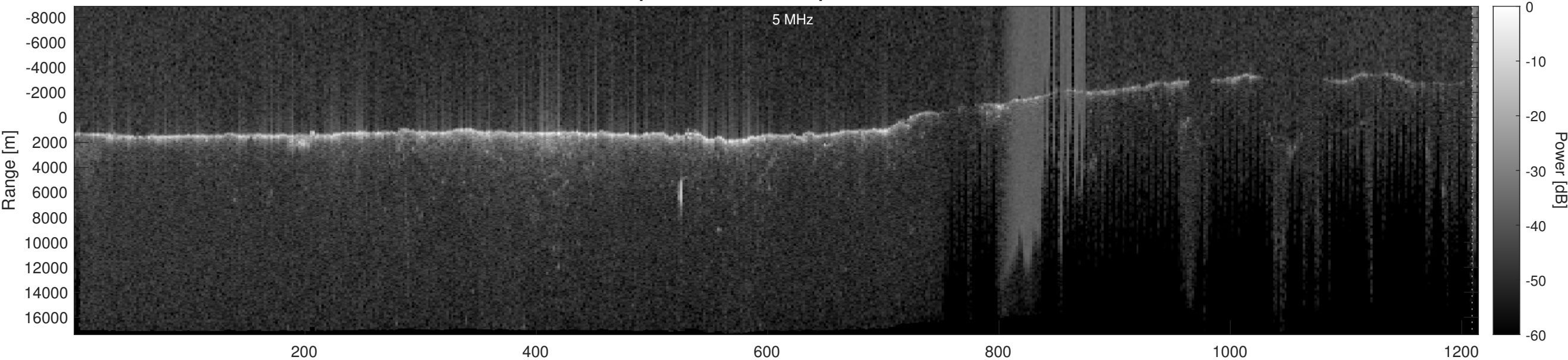
Orbit 11488, Optimized, Window, Depth-Corrected, Channel 2
