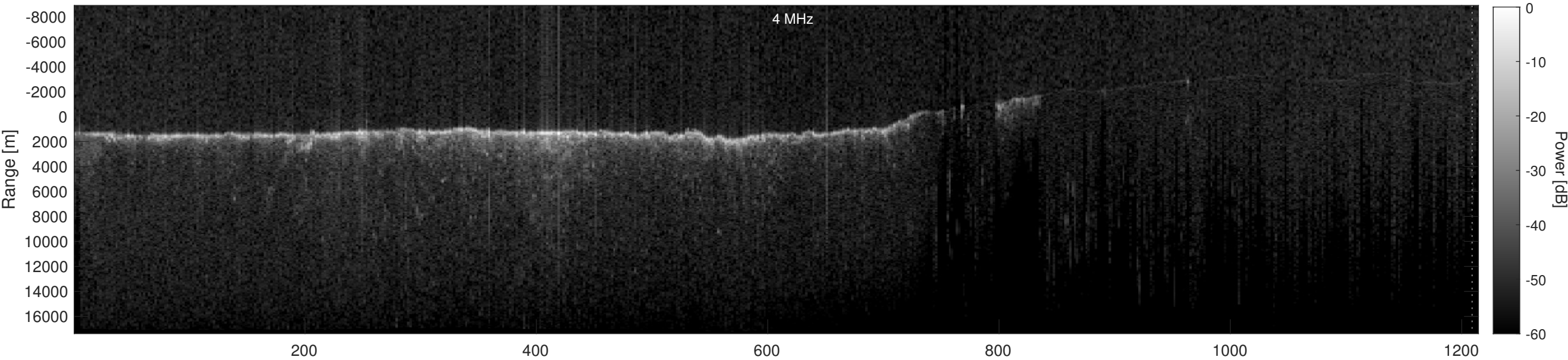
Orbit 11488, Depth-Corrected Cluttergram
