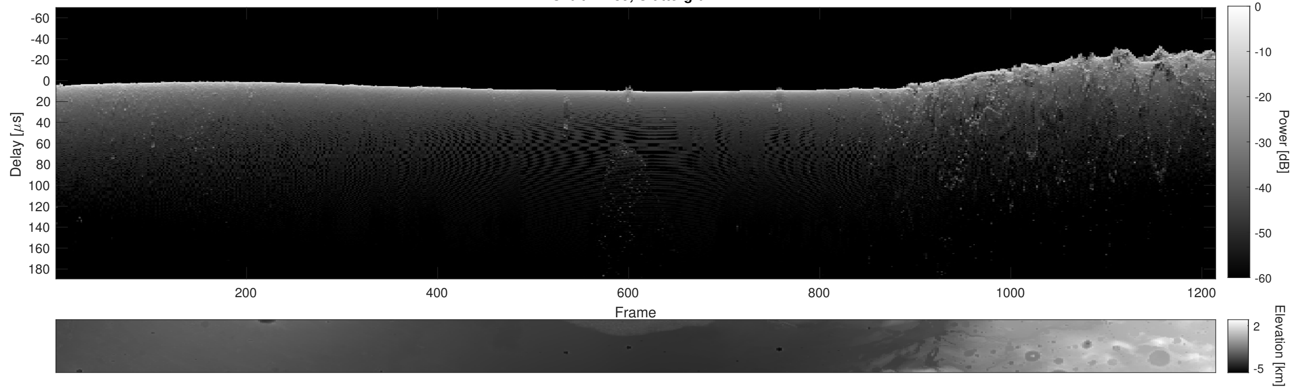
Orbit 11489, Cluttergram
