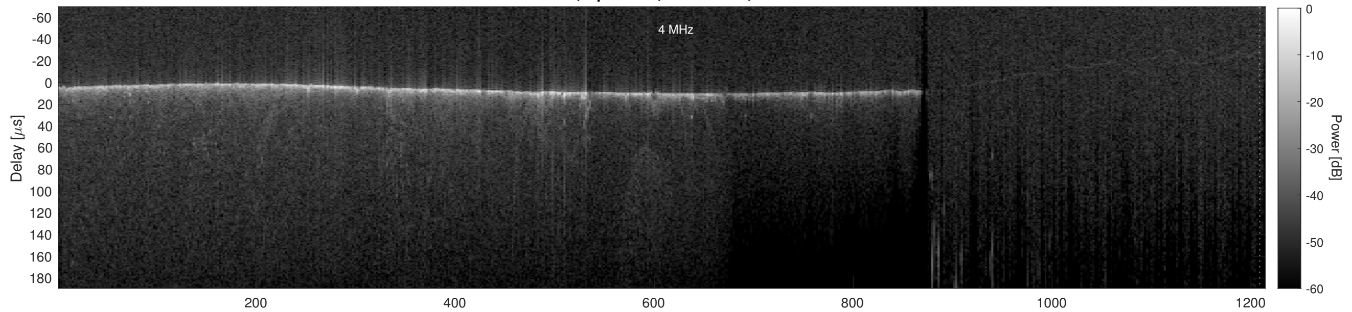
Orbit 11489, Cluttergram
