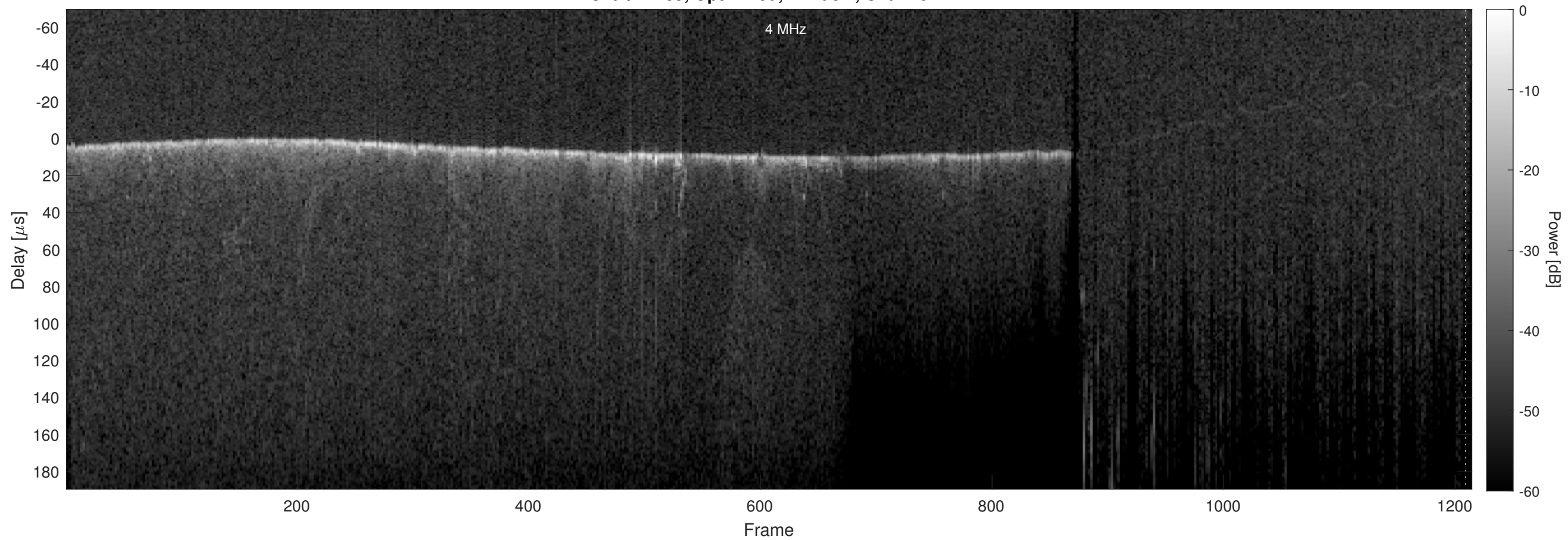
Orbit 11489, Optimized, Window, Channel 2
