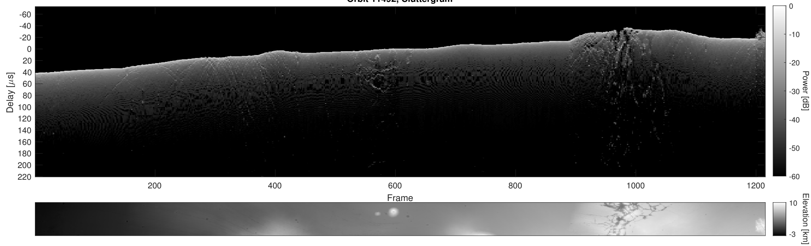
Orbit 11492, Cluttergram
