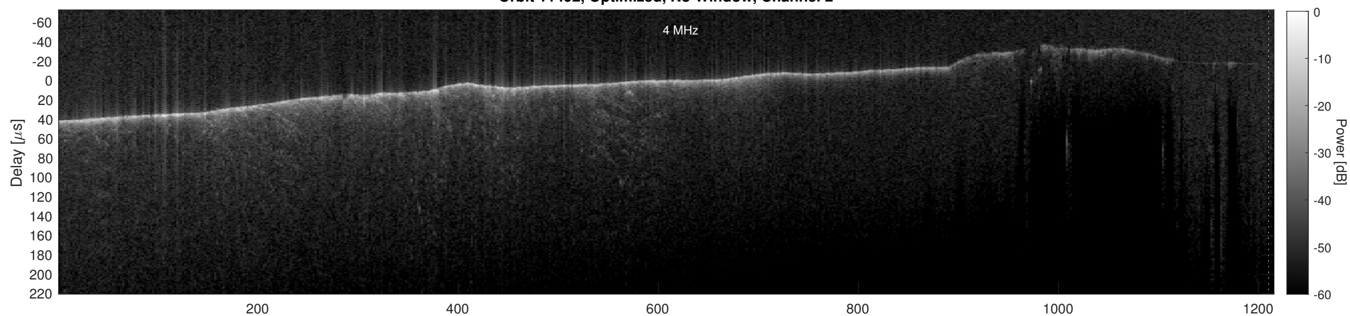
Orbit 11492, Cluttergram
