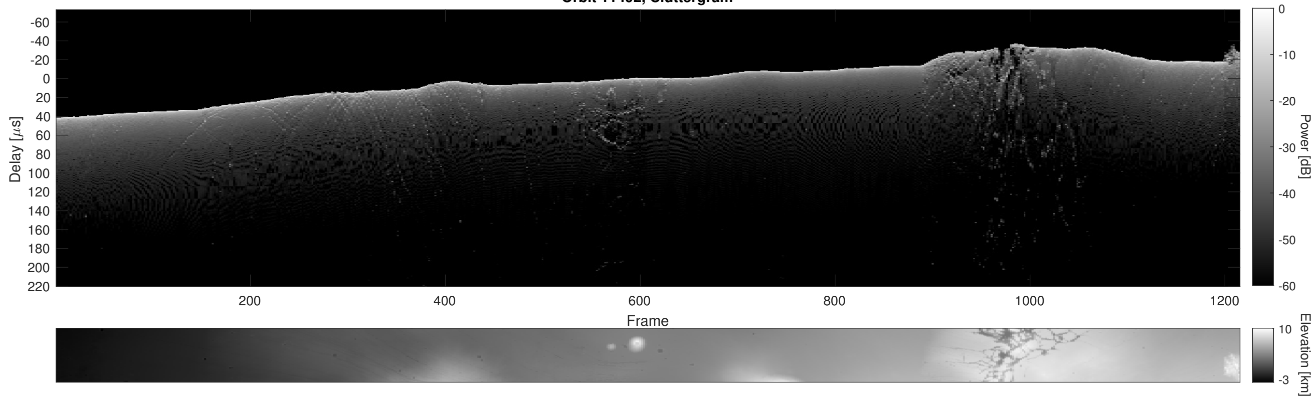
Orbit 11492, Cluttergram
