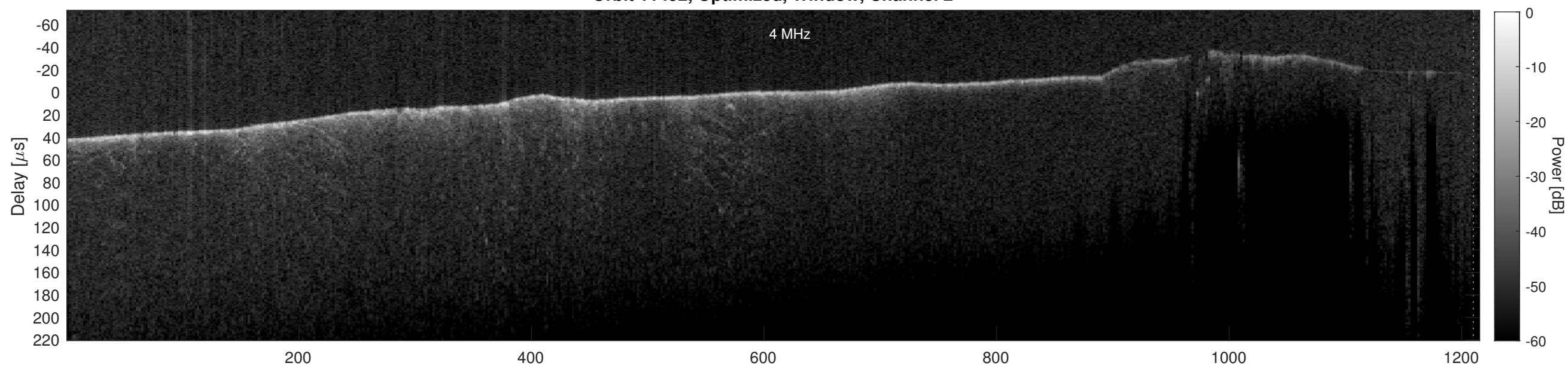
Orbit 11492, Cluttergram
