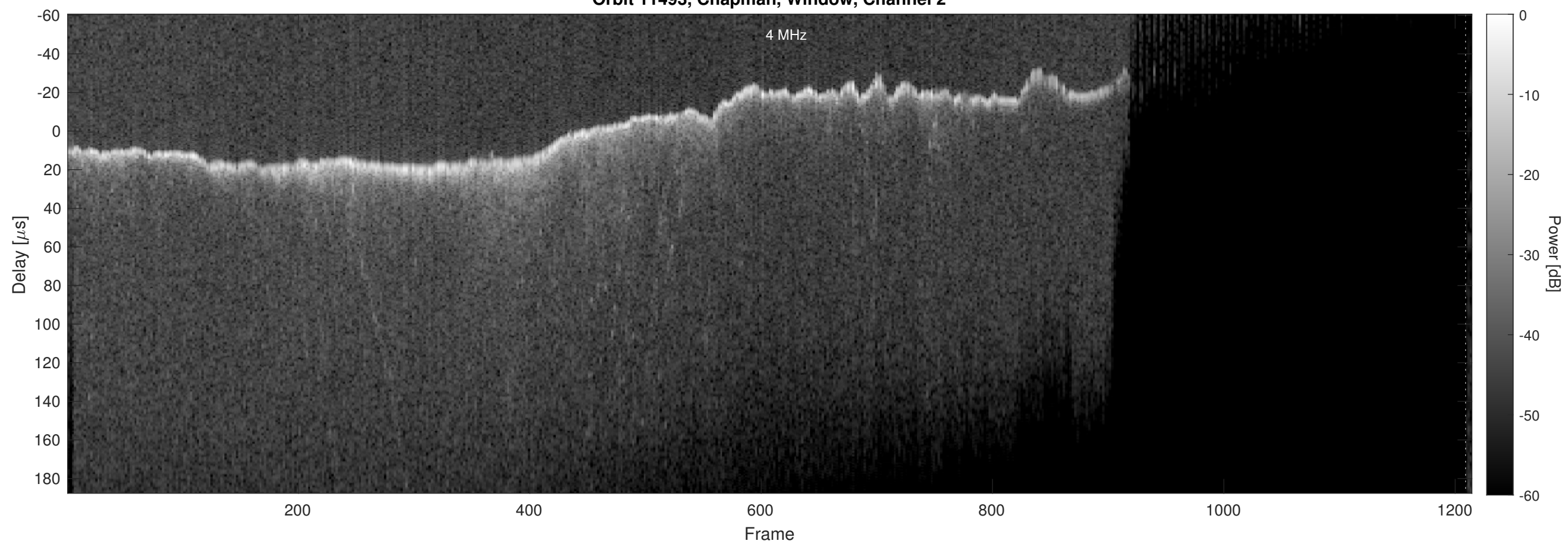
Orbit 11493, Chapman, Window, Channel 2
