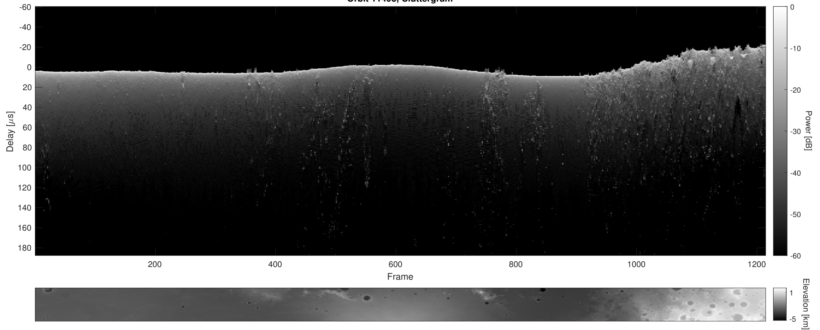
Orbit 11493, Cluttergram
