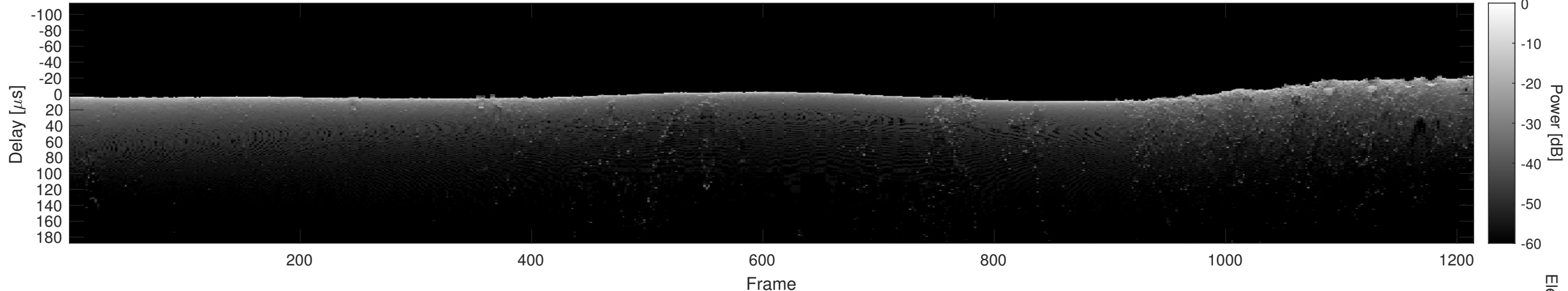
Orbit 11493, Cluttergram
