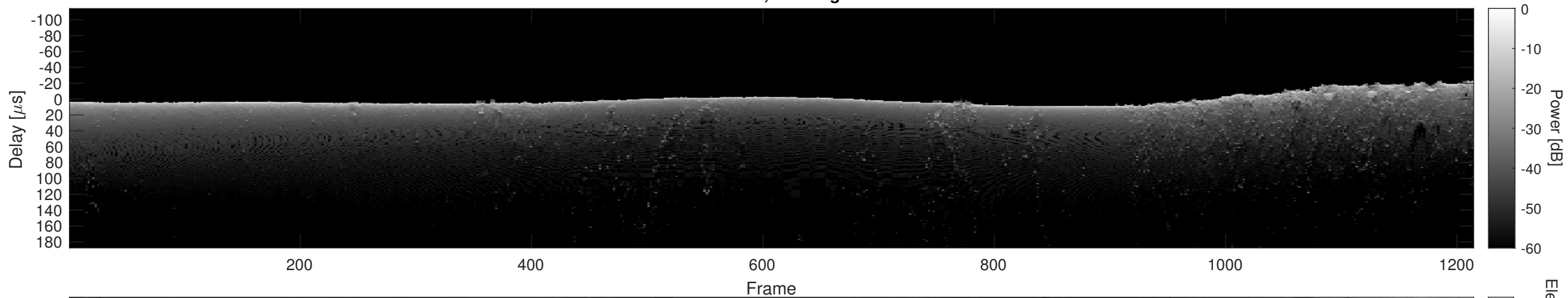
Orbit 11493, Cluttergram
