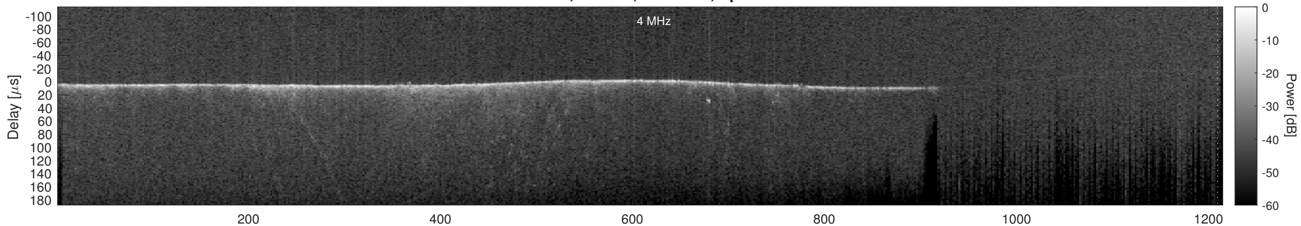
Orbit 11493, Cluttergram
