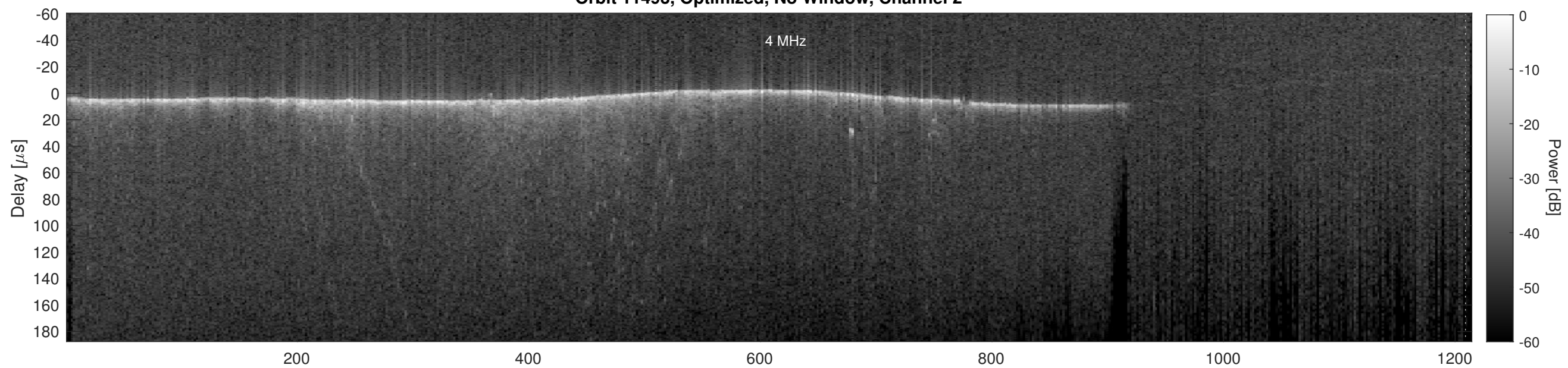
Orbit 11493, Cluttergram
