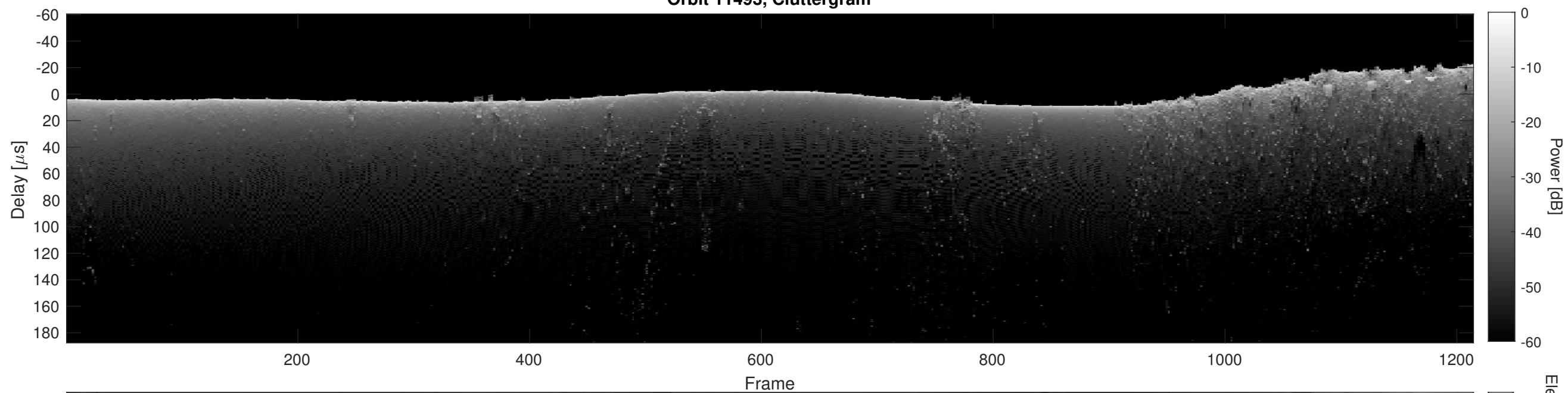
Orbit 11493, Cluttergram
