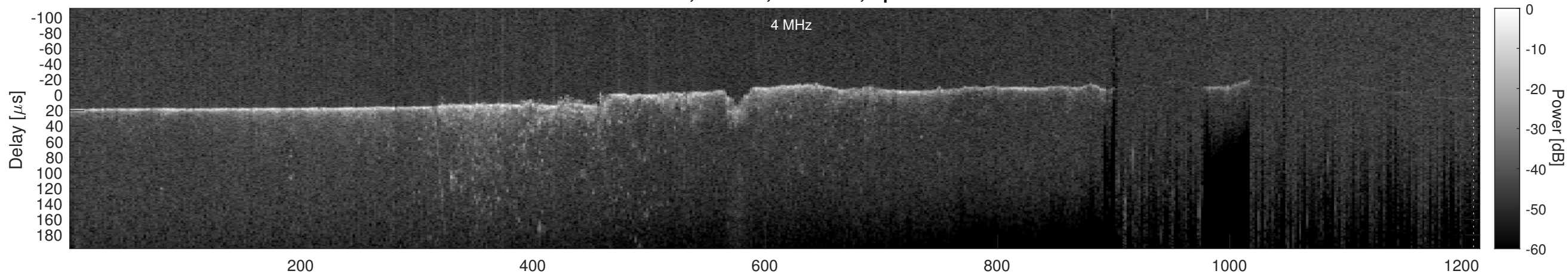
Orbit 11494, Cluttergram
