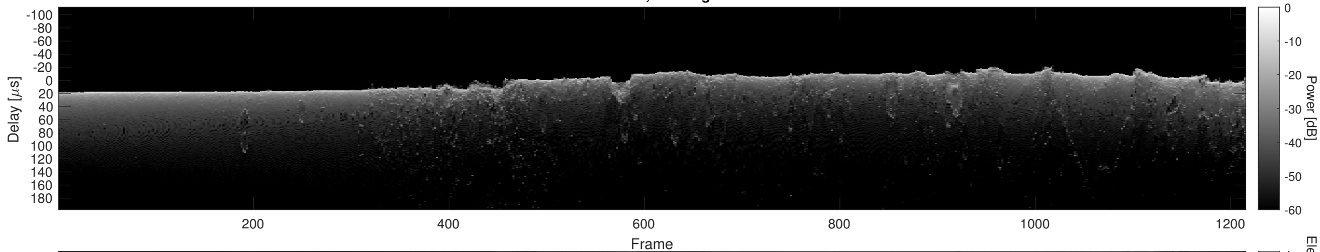
Orbit 11494, Cluttergram
