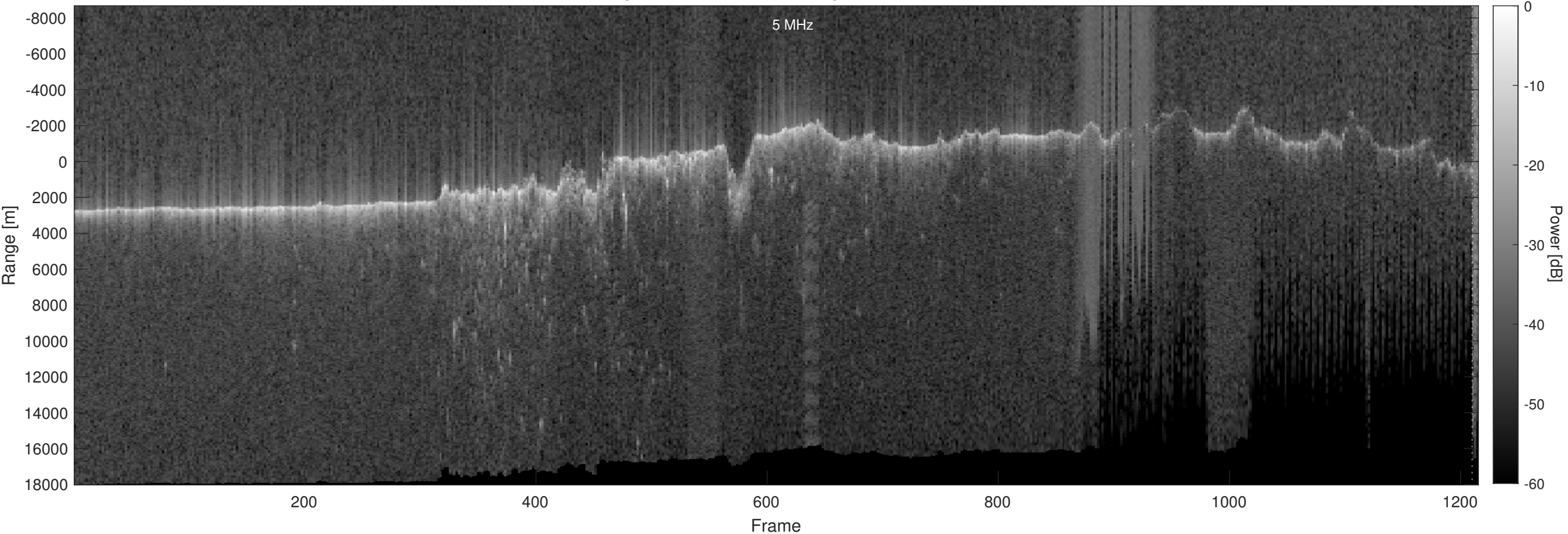
Orbit 11494, Optimized, No Window, Depth-Corrected, Channel 2
