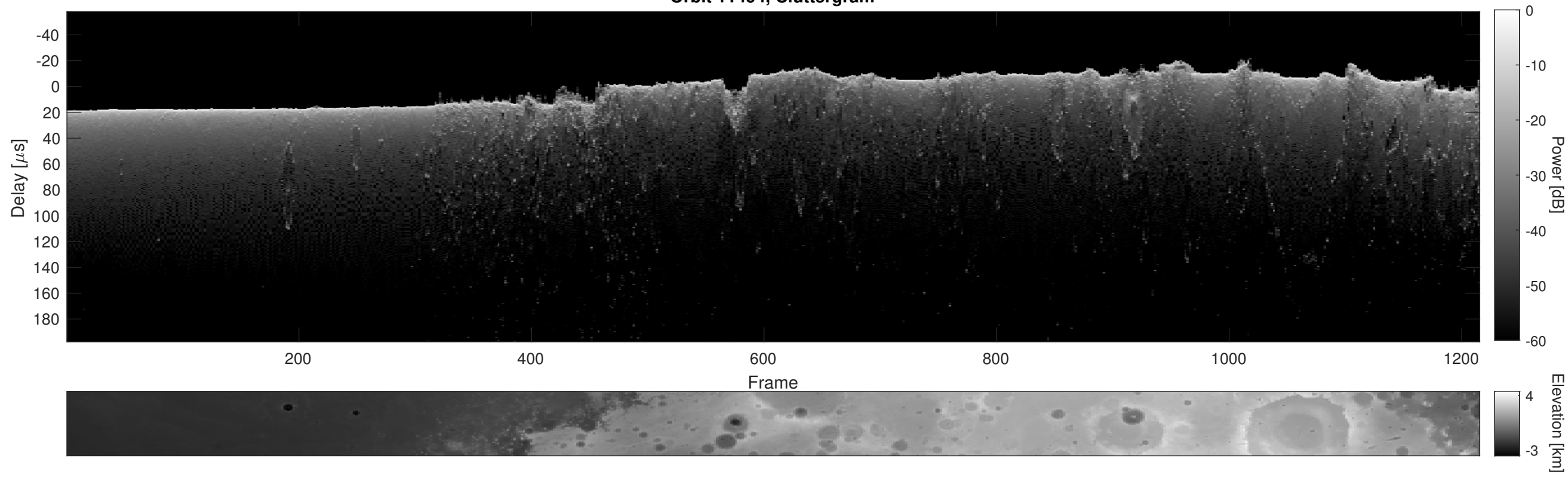
Orbit 11494, Cluttergram
