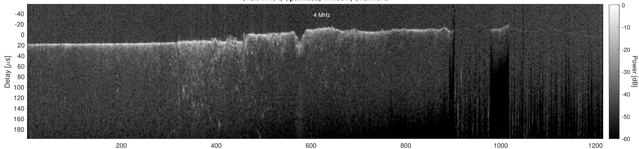
Orbit 11494, Cluttergram
