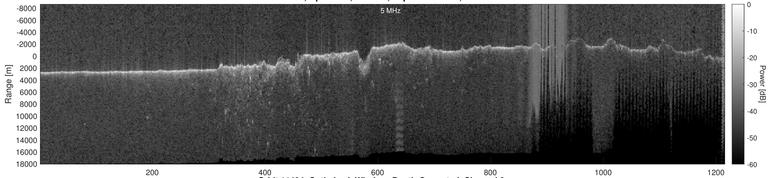
Orbit 11494, Optimized, Window, Depth-Corrected, Channel 2
