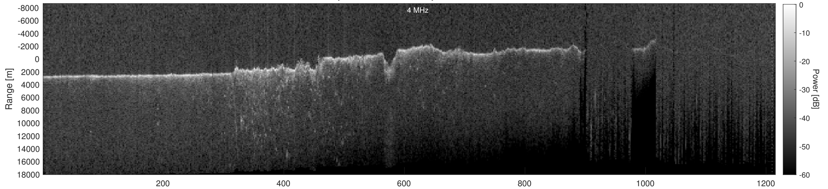
Orbit 11494, Depth-Corrected Cluttergram
