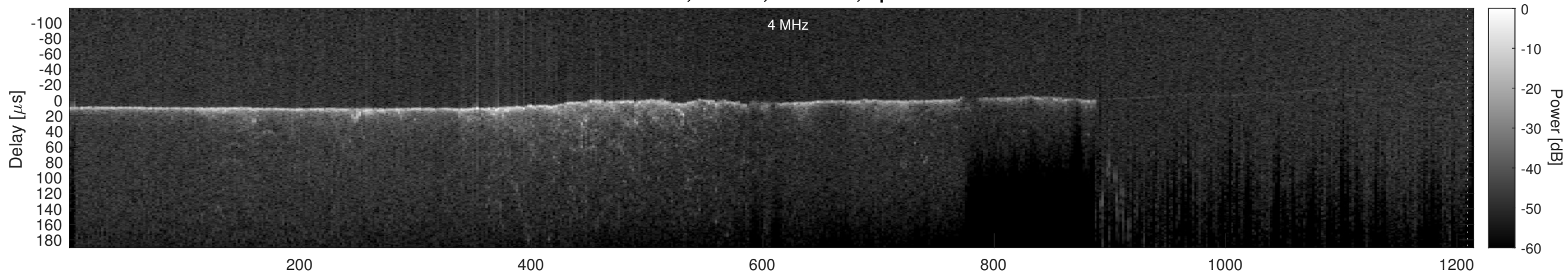
Orbit 11498, Cluttergram
