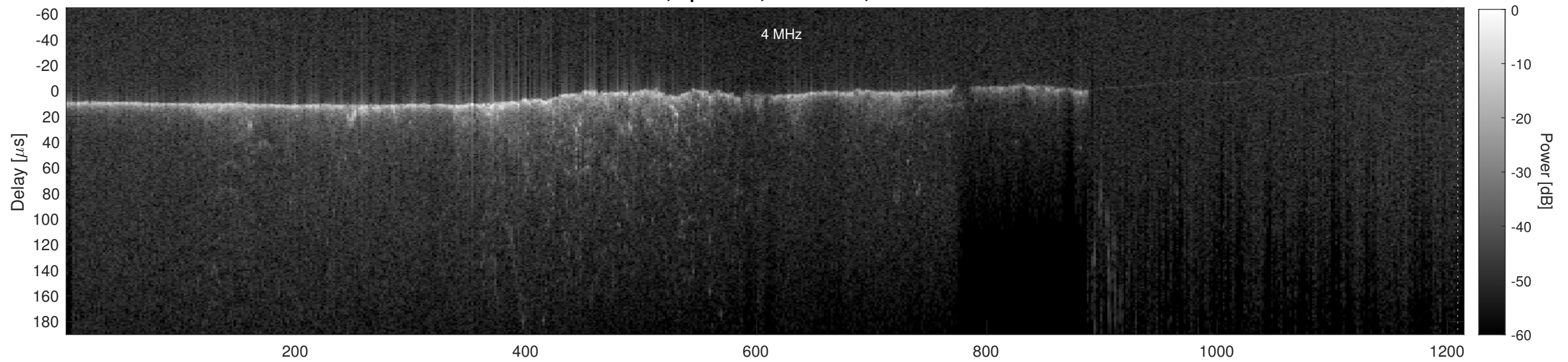
Orbit 11498, Cluttergram
