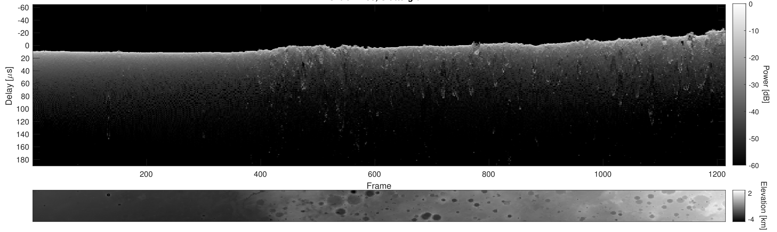
Orbit 11498, Cluttergram
