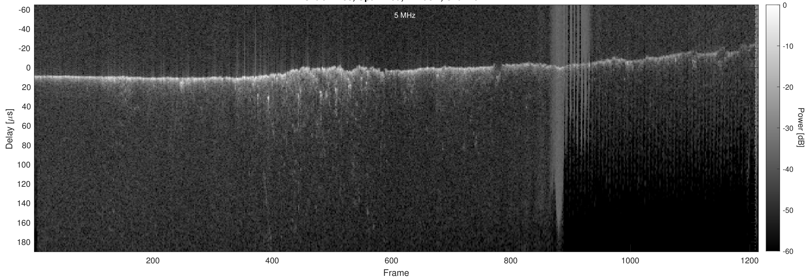
Orbit 11498, Optimized, Window, Channel 2
