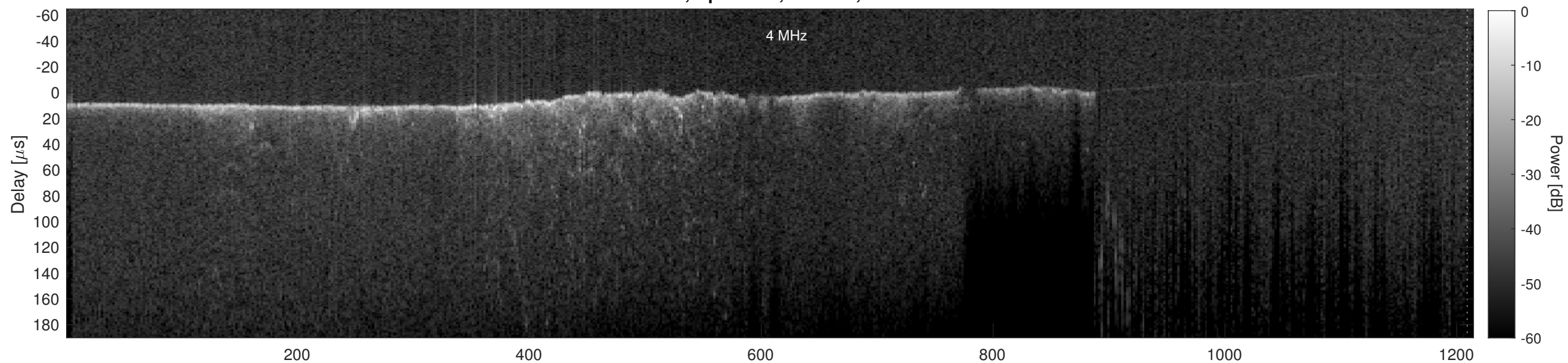
Orbit 11498, Cluttergram
