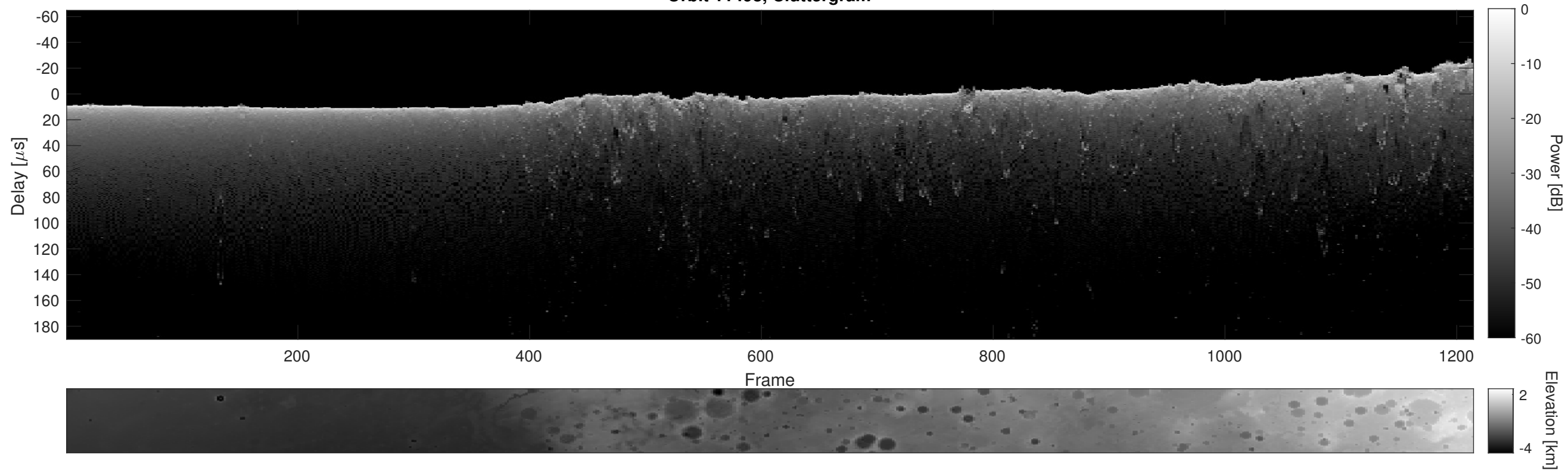
Orbit 11498, Cluttergram
