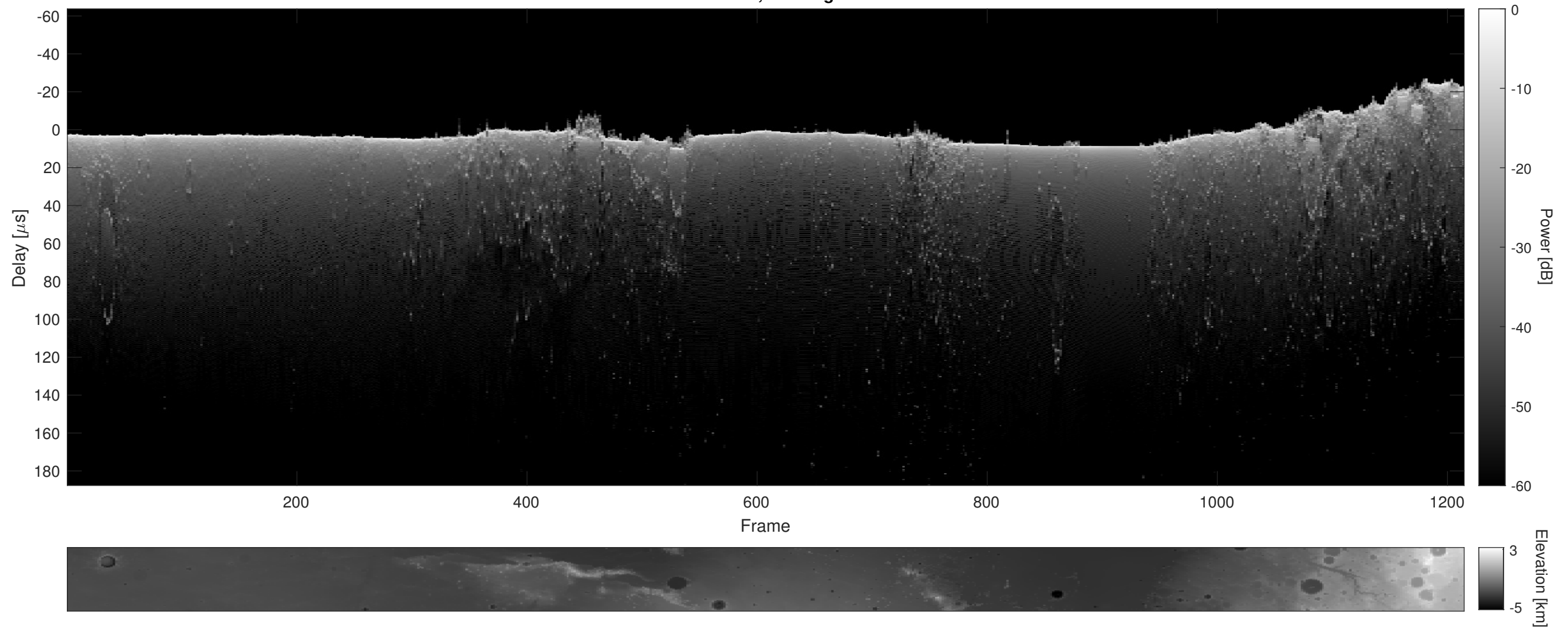
Orbit 11500, Cluttergram
