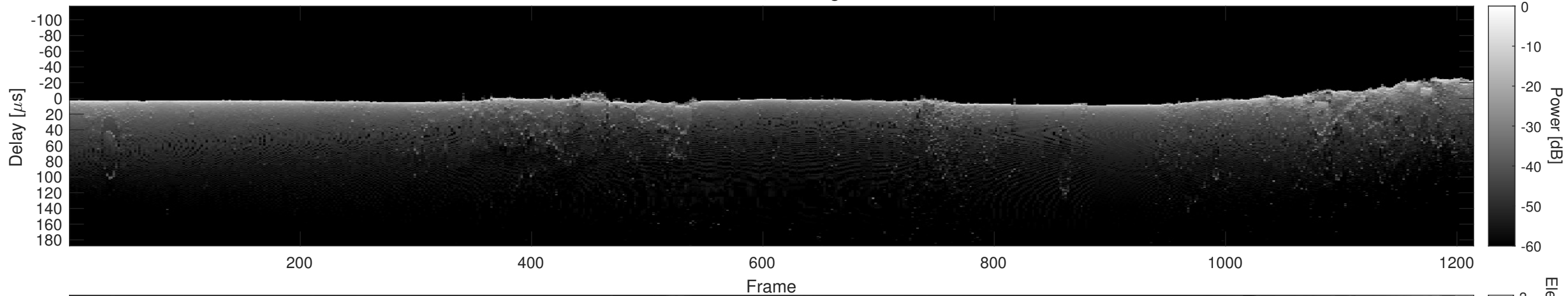
Orbit 11500, Cluttergram
