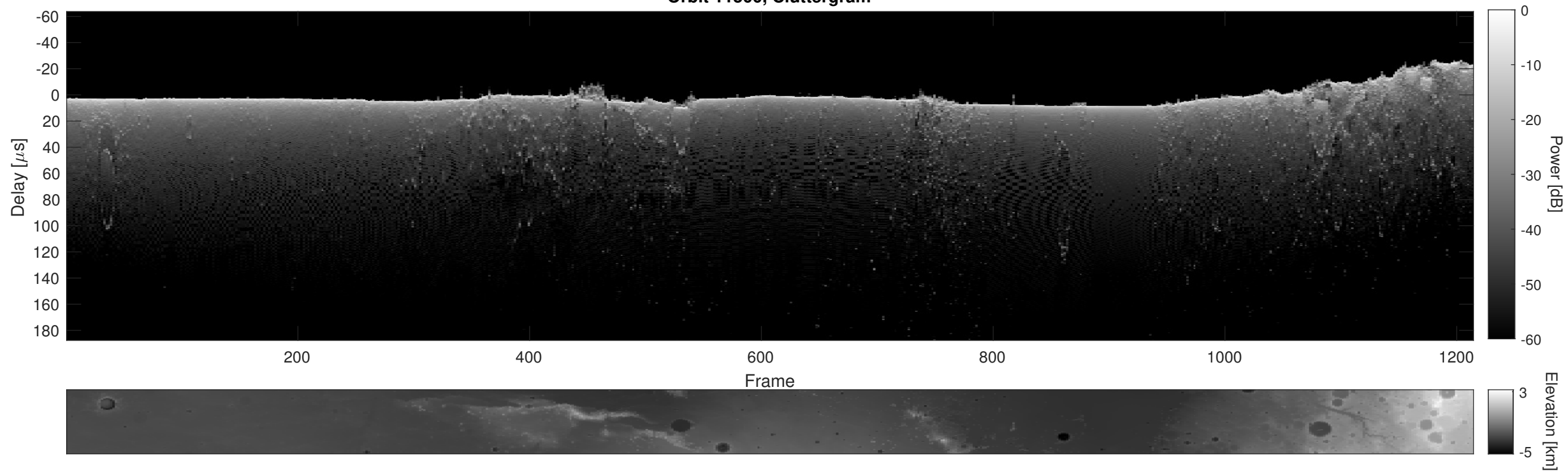
Orbit 11500, Cluttergram
