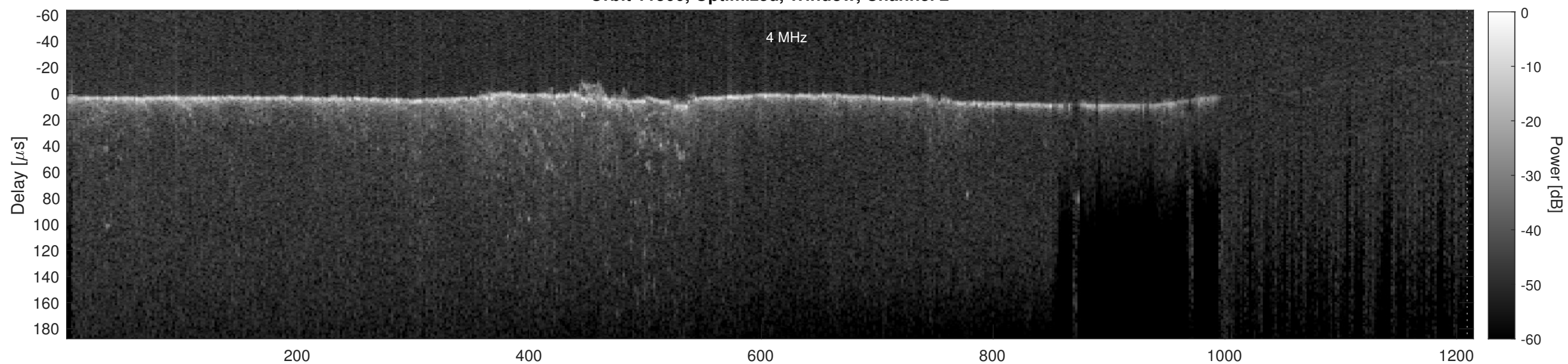
Orbit 11500, Cluttergram
