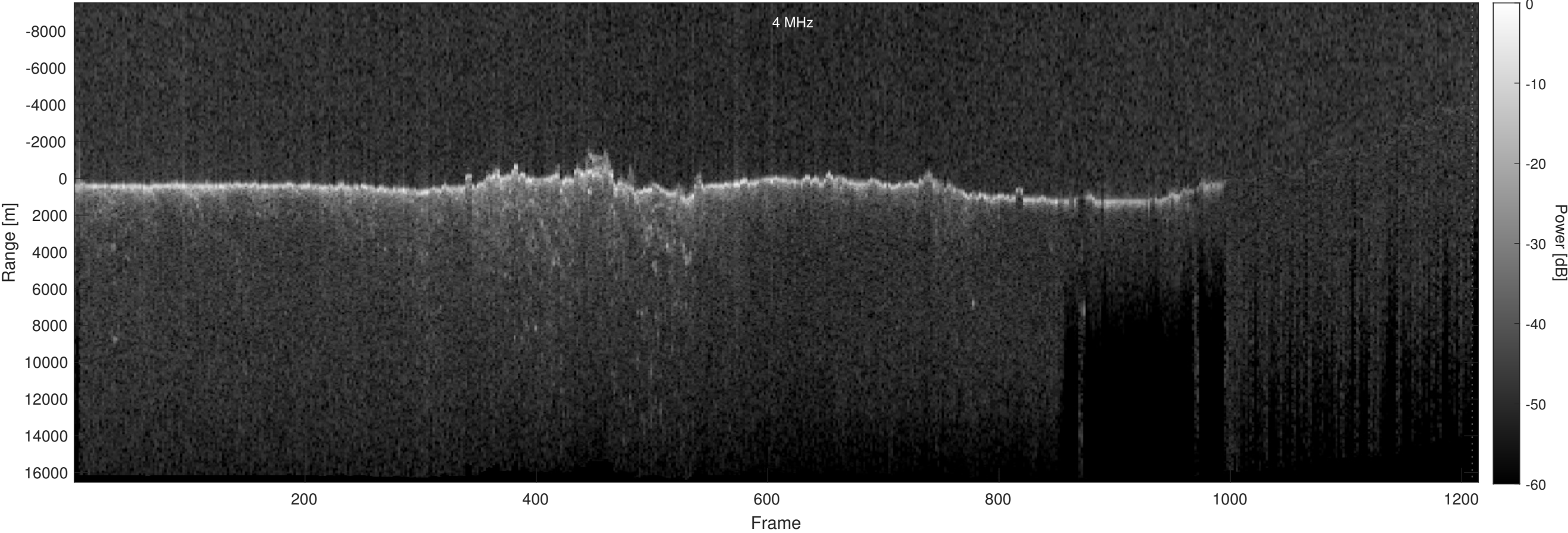
Orbit 11500, Optimized, Window, Depth-Corrected, Channel 2
