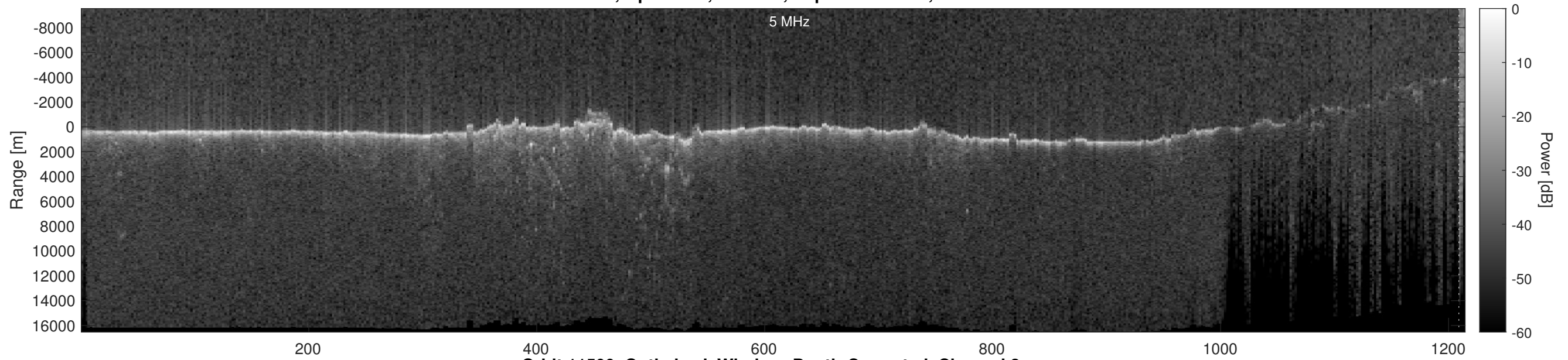
Orbit 11500, Optimized, Window, Depth-Corrected, Channel 2
