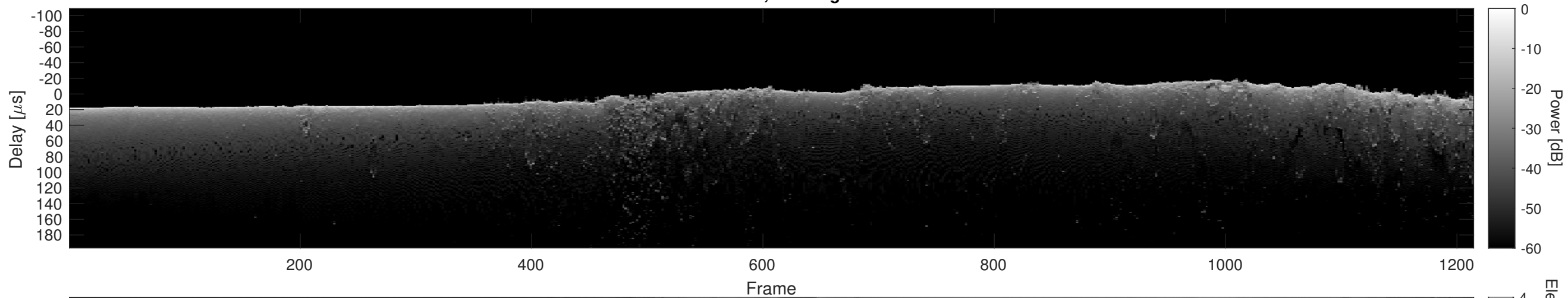
Orbit 11501, Cluttergram
