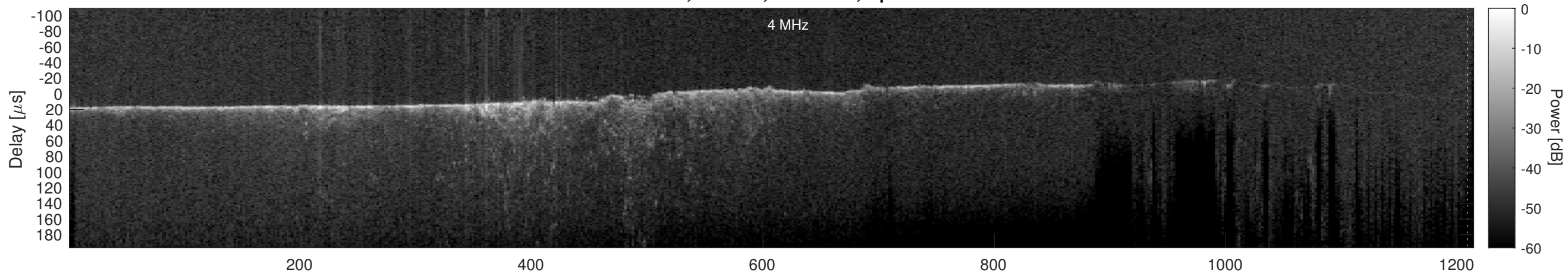
Orbit 11501, Cluttergram
